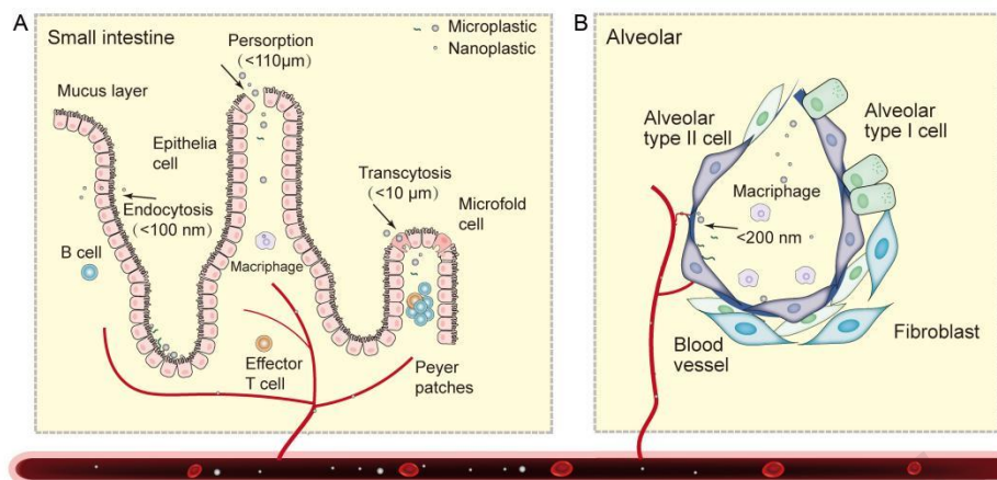
Figure 1. The possible absorption, transfer and accumulation mechanisms of micro- and nanoplastics in human intestines (A) and lungs (B).
