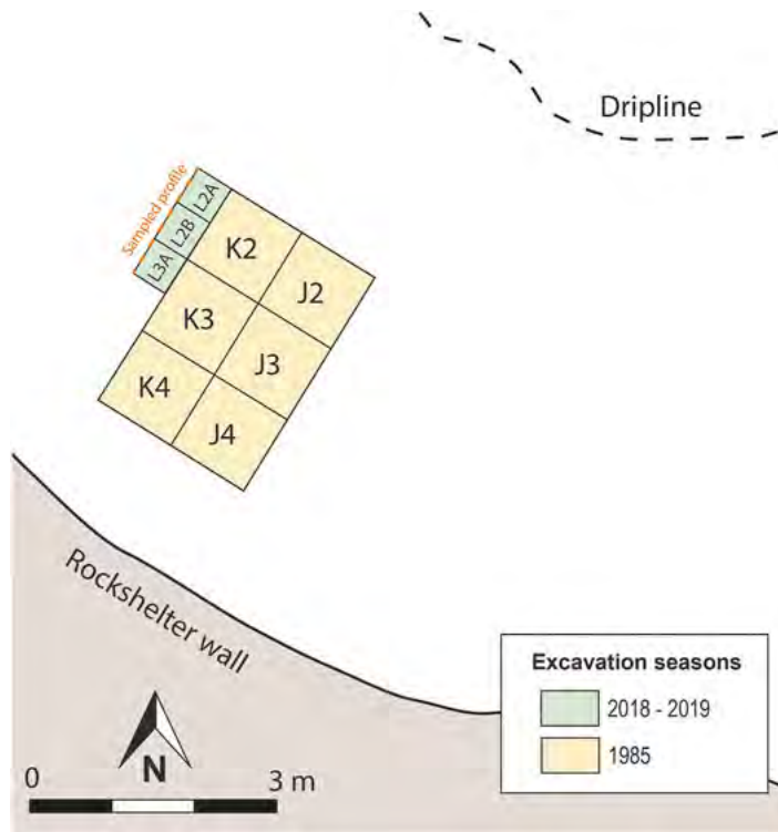
Figure 3.3: Umhlatuzana site map illustrating the excavation squares of the different fieldwork campaigns.
