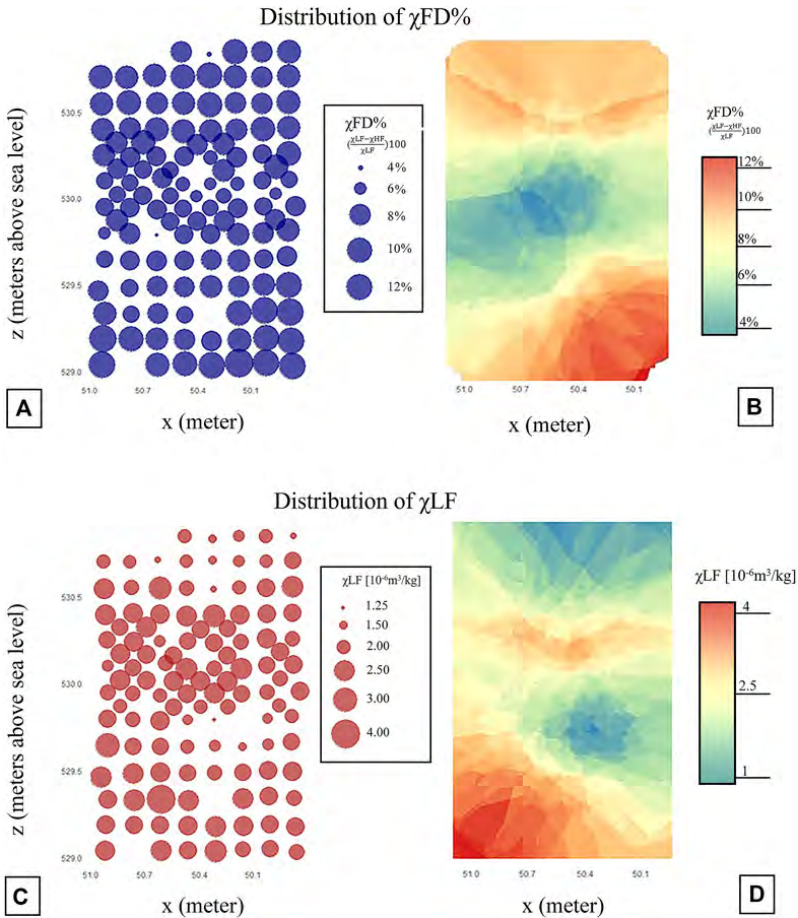
Figure 3.8: A. \chi_{FD\%} bubble plot. B. \chi_{FD\%} heat map. C. \chi_{LF} bubble plot. D. \chi_{LF} heat map.
