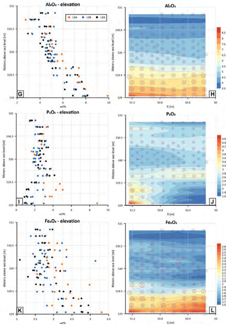
Figure 3.6: Results for selected elements. A. \text{SiO}_2 elevation plot. B. \text{SiO}_2 contour map. C. CaO elevation plot. D. CaO contour map. E. CL elevation plot. F. Cl contour map. XRF results for selected elements. G. \text{Al}_2\text{O}_3 elevation plot. H. \text{Al}_2\text{O}_3 contour map. I. \text{P}_2\text{O}_5 elevation plot. J. \text{P}_2\text{O}_5 contour map. K. \text{Fe}_2\text{O}_3 elevation plot. L. \text{Fe}_2\text{O}_3 contour map.
