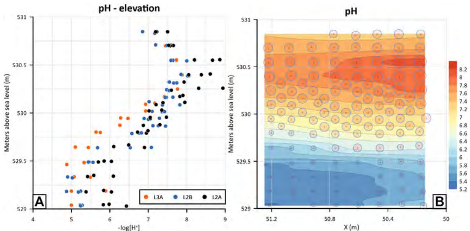
Figure 3.5: Results from the grid-based pH analysis illustrated using an elevation plot (A) and contour map (B).
