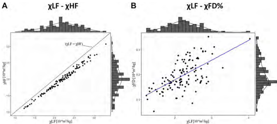
Figure 3.7: A. Plot of \chi_{LF} and \chi_{HF} values, with the distribution of values represented along the margins. The predictive model represents the expected distribution of \chi_{LF} = \chi_{HF} . B. Plot of \chi_{LF} and \chi_{FD} values with distribution represented along the margins and liner model demonstrating the relationship between the values.
