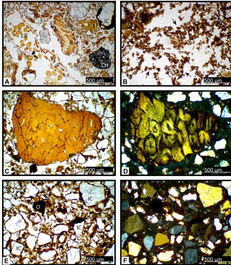
Figure 3.9: Photomicrographs of sedimentary components identified in micromorphology thin sections.
