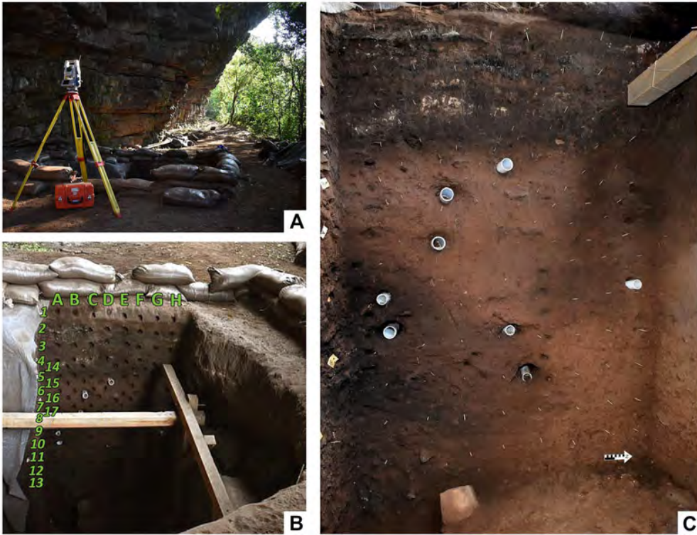
Figure 3.2: A View of Umhlatuzana rockshelter. B Overview of the western profile after the grid-based bulk sediment sampling. C West profile of squares L3A, L2B, L2A with grid-based sample locations. The northern part of the profile is affected by shading from the safety scaffolding installed in the excavation pit.
