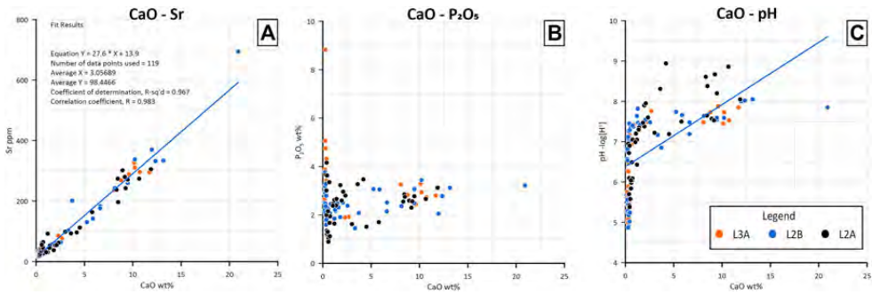
Figure 3.10: Correlation plots for CaO–Sr (A), CaO–P 2 O 5 (B), and CaO–pH (C).
