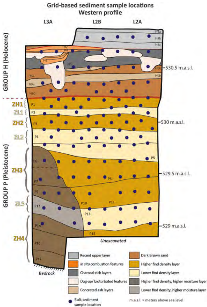
Figure 3.4: Stratigraphic drawing of the western profile based on Sifogeorgaki et al. (2020) highlighting the location of distinct lower and higher find density zones as well as the grid-based sampling locations of the current study.
