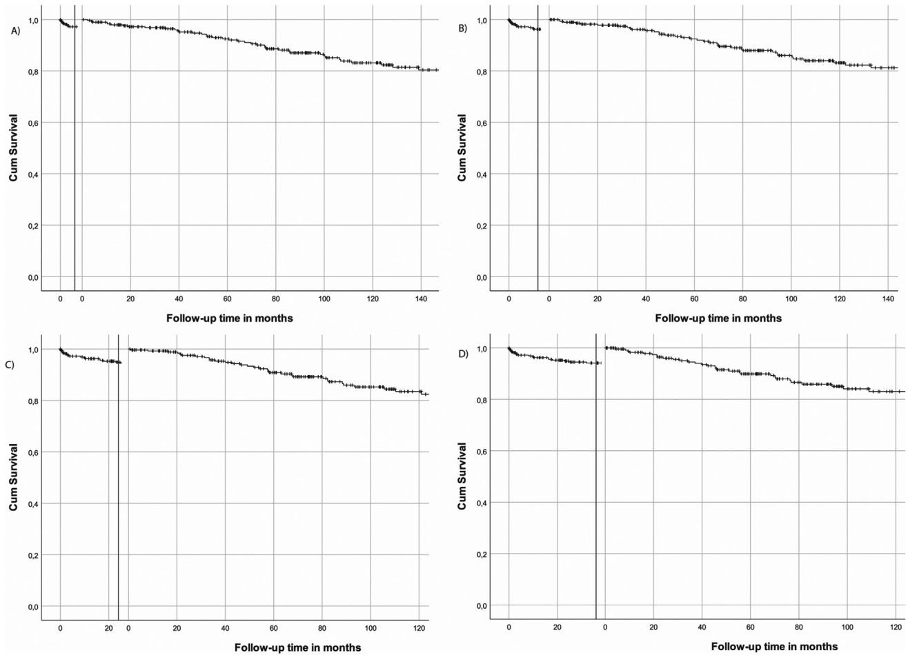
Supplementary Figure 1. The relation between the used landmark analysis at (A) 6 months, (B) 12 months, (C) 24 months, and (D) 36 months and transplant-free survival. The black vertical line represents the landmark.
