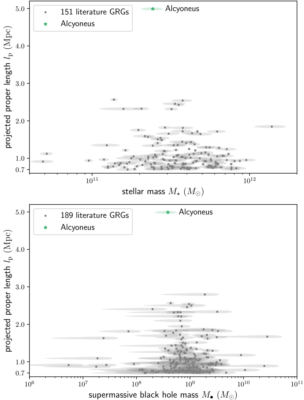
Figure 4.7: Relations between the GRG projected proper length l_p and the host galaxy stellar mass M_* (top panel) and between the GRG l_p and the host galaxy SMBH mass M_\bullet (bottom panel). Our methods allow these properties to be determined for a small proportion of all literature GRGs only. Literature GRGs are marked with grey disks, and Alcyoneus is marked with a green star. Translucent ellipses indicate -1 to +1 standard deviation uncertainties. Alcyoneus’s host has a below-average stellar mass (percentile 25 \pm 9\% ) and SMBH mass (percentile 23 \pm 11\% ).
