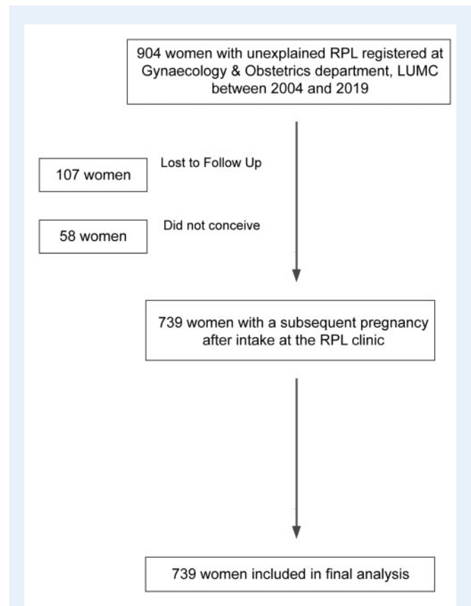
Figure 1. Flow chart of women with unexplained recurrent pregnancy loss who were considered for inclusion in external the validation.
