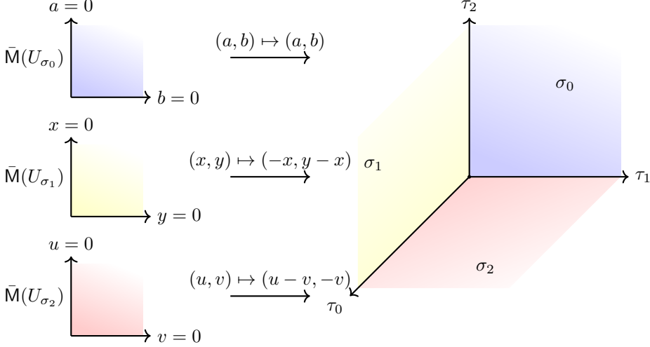
Figure 2.4: Visualisation of the interactions of the characteristic monoid sheaves in \mathbb{P}_k^2 .
