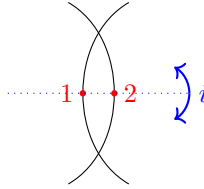
Figure 2.16: Automorphism i
