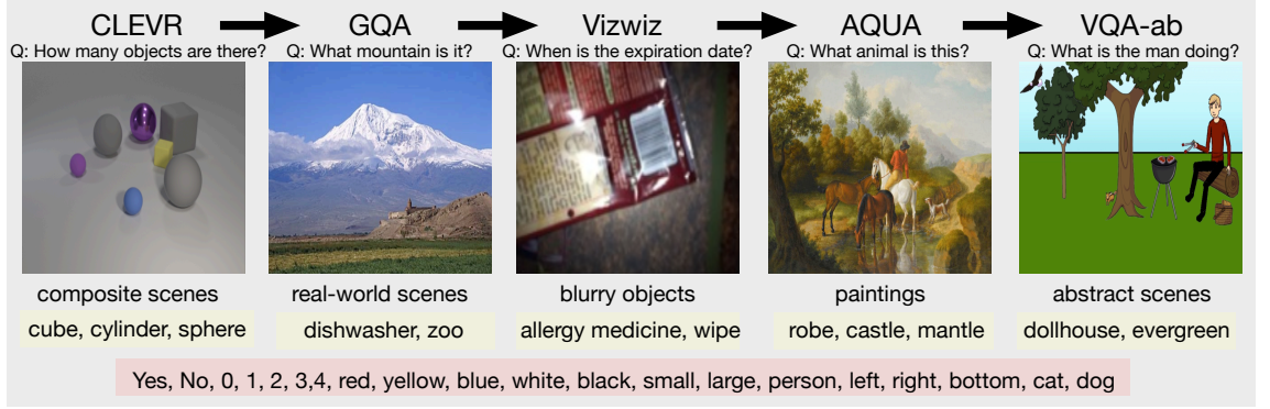
Figure 1.5: Our MDL-VQA benchmark involves five VQA tasks in the visual domains of composite, realistic, blurry-objects, artistic and abstract scenes. Unlike standard domain-incremental learning, the label spaces for different domains are inconsistent, where words in red shading denote some general answers coexist in several domains, and in yellow shading are domain specific.
