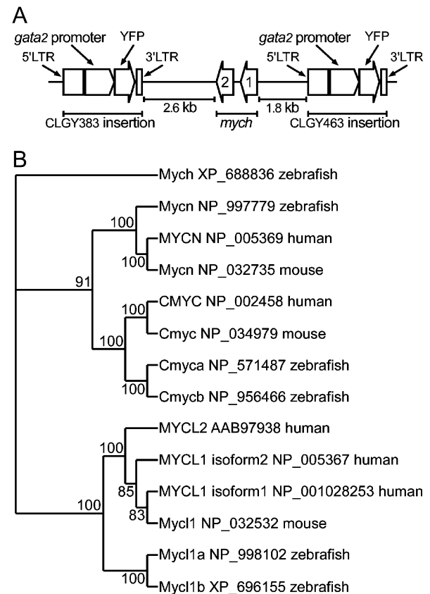
Fig. 2 Association of the CLGY463 insertion with a member of the myc gene family. (A) Genomic organization of the myc gene on chromosome 6 and orientation of the upstream viral insertion in transgenic line CLGY463, consisting of 5' and 3' LTRs (long terminal repeats), a basal gata2 promoter and a YFP reporter gene. In addition, the orientation of the viral insertion in transgenic line CLGY383 is shown. (B) Unrooted phylogenetic tree based on ClustalW alignment of the full-length human, mouse and zebrafish Myc proteins. The numbers indicate the occurrence of nodes during bootstrap analysis, given as percentages of 10,000 reiterations. Human MYCL2 is derived from a pseudogene. Genbank accession numbers of reference sequences used for the alignment are indicated in the figure.
