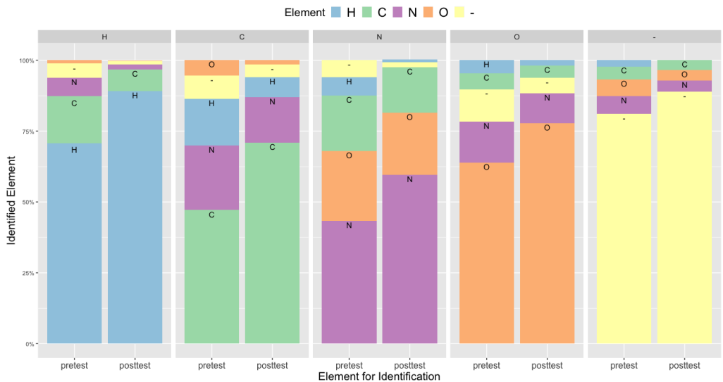
Figure 5.5: Stack diagram depicting the percentages of correct identifications and misidentifications of elements during the experiment, ordered from low to high atomic mass.
