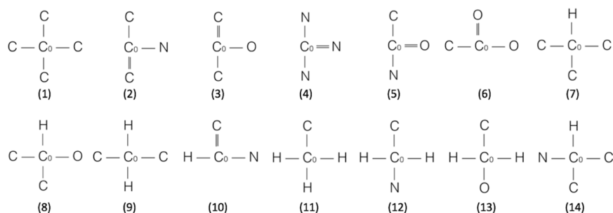
Figure 5.2: 14 structural formulas for Validation 1.
