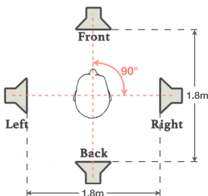
Figure 4.2: Implementation of the four speakers setup.
