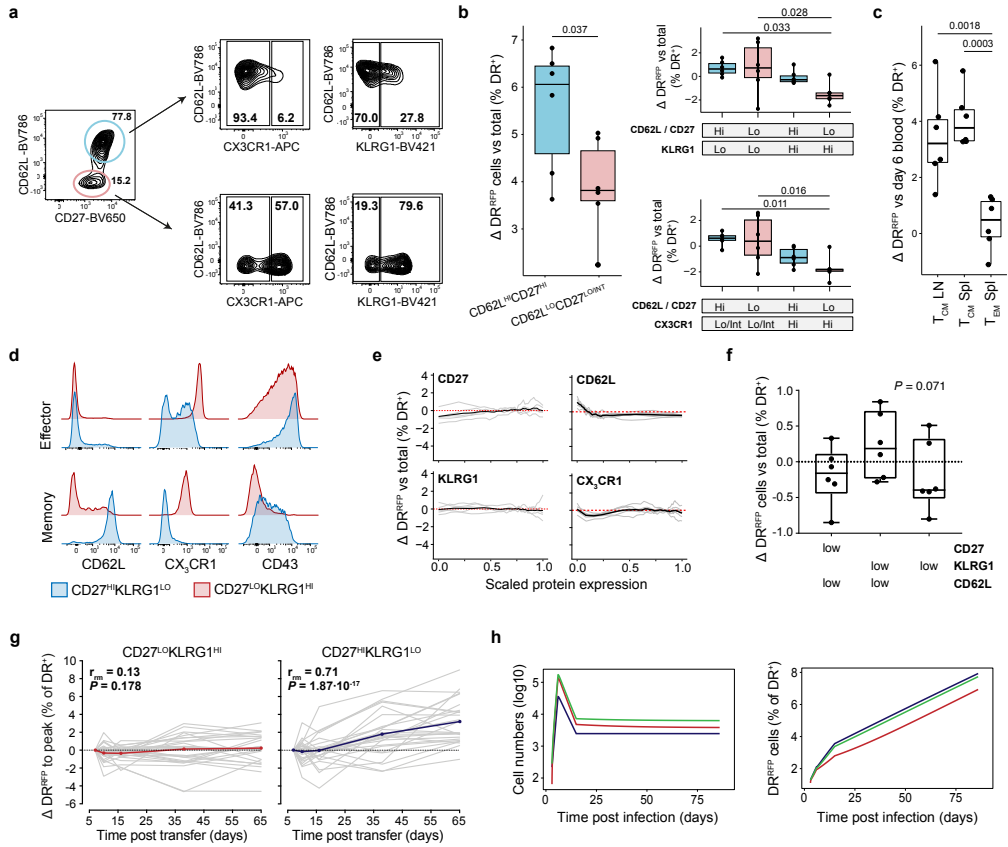
Extended Data Fig. 2. Evaluation of the division history of T cell subsets throughout a response to Lm -OVA.
