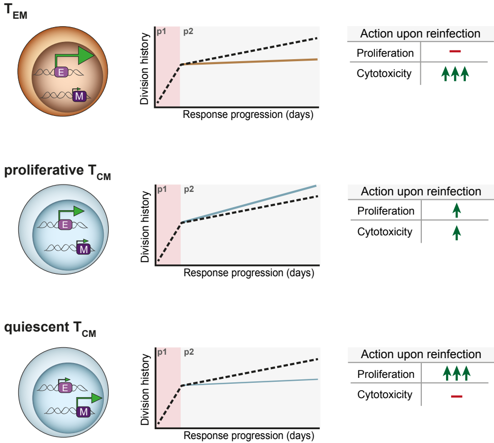
Extended Data Fig. 9. Model describing replicative behaviors in the CD8 + memory T cell pool. Upon infection, antigen-specific CD8 + T cells activate and rapidly expand (phase 1, p1). Following pathogen clearance (p2), a subset of memory T cells continues to divide, resulting in a progressive increase in the replicative history of the overall T cell memory pool (dotted line). Within this population, three separate behaviors of transcriptionally disparate memory T cell pools can be distinguished. Top ) Terminally differentiated T EM cells that cease division after the inflammation phase (p1) and that are marked by high transcription of effector- and minimal expression of multipotency-associated genes ([E], [M]). Upon reactivation, these cells exert rapid effector functions, but lack the potential to re-expand. Middle ) A subgroup of T CM that continues to proliferate in the memory phase, exhibits diminished levels of multipotency-associated transcripts, and that abundantly expresses effector-associated genes. Although the functionality of these cells upon reinfection requires further study, their heightened expression of effector-associated genes suggests that these cells exert cytotoxic activity upon reinfection. The contribution of these cells to the secondary T EFF pool is limited. Bottom ) A subgroup of T CM cells that shows low expression of effector-associated genes but increased expression of multipotency-associated genes, and that exists in a near-quiescent state after the inflammation phase. Upon renewed infection, this cell pool is primarily responsible for the generation of a new wave of secondary T EFF . Based on their transcriptional profile, these cells are expected to have limited immediate cytotoxic functions.
