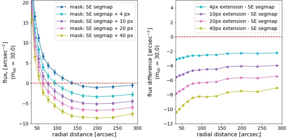
Figure 4.A.1: Left: surface brightness (SB) profiles of group central galaxies (CG) beyond 50'' with different levels of mask-extension (as shown in the top-right corner). Compared to the original segmentation map (blue), the 4, 10, 20, and 40-pixel extended masks to sources other than CG produce monotonically lower flux profiles. Error bars show the 1\sigma error to the corresponding mean values. Right: change of measured SB profiles of the stacked BGGs. Different lines here show the difference between different levels of mask extension (as shown in the top-right corner) compared to the initial mask obtained from the segmentation map of SExtractor. The main noticeable feature from both the panels is that, even with a 4-pixel (about 1.3 kpc) extension to the segmentation map, the outer profile is lowered by about 3 ADU compared to the original mask from the segmentation map.
