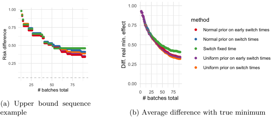
Figure S7.2: Example of a confidence sequence and average difference from upper bound to true minimal effect size through 100 simulations, for different switch priors on j^* . 30 observations were made in each stratum, and the real differences were 0.5, 0.4 and 0.05. For the priors on early switch times, all prior mass was distributed between batch numbers 5 up to 10. \alpha was set to 0.05.
