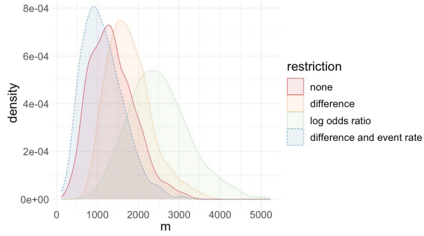
(b) Simulated stopping times in setting with continuing until E \geq 20
