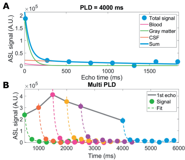
Figure 3.2. Example of single-voxel data fitted to the triexponential model. A shows the separation of the signal into three exponentials with T_2 = 60 ms (GM), 150 ms (blood), and 1500 ms (CSF) for a single time point. B shows the fit to the sum of these three exponential components for all time points. Note that there are no error-bars as this dataset provided a single value for each voxel (any averaging over shots was done in image reconstruction).
