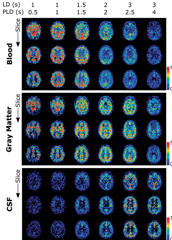
Figure 3.6. Results of triexponential fit in subject 1. The signal originating from each of the three compartments is shown separately (note that because the CSF signal is much lower, a different scale is used). Maps are given for three slices, one intersecting the circle of Willis (top), one intersecting the choroid plexus (middle) and one higher in the brain (bottom). Different time points are shown with increasing LD/PLD from left to right.
