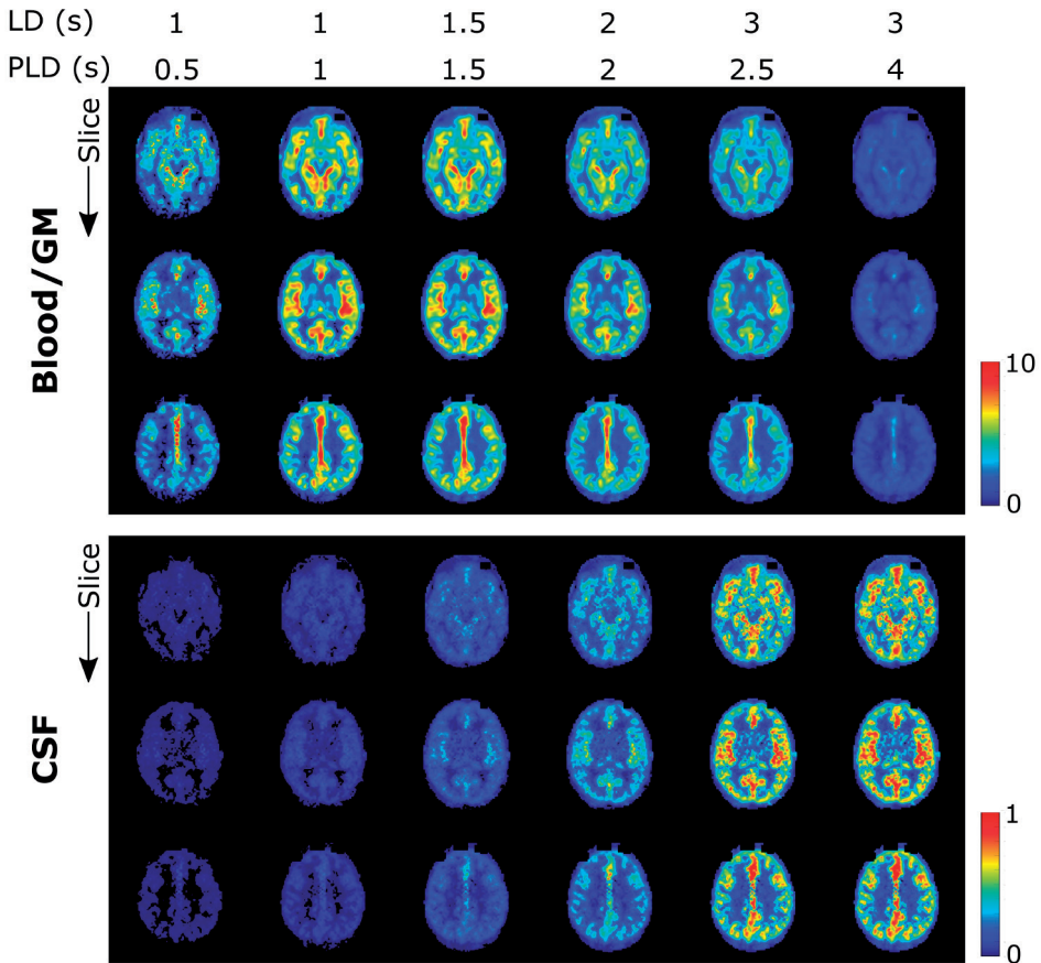
Figure 3.10. Reconstructed blood (+ GM) and CSF fractions from the fitted parameters of Figure 3.7, simulating the signal at all experiment time points for an artificial echo time of 0 ms. Note the different scaling of the CSF fraction.
