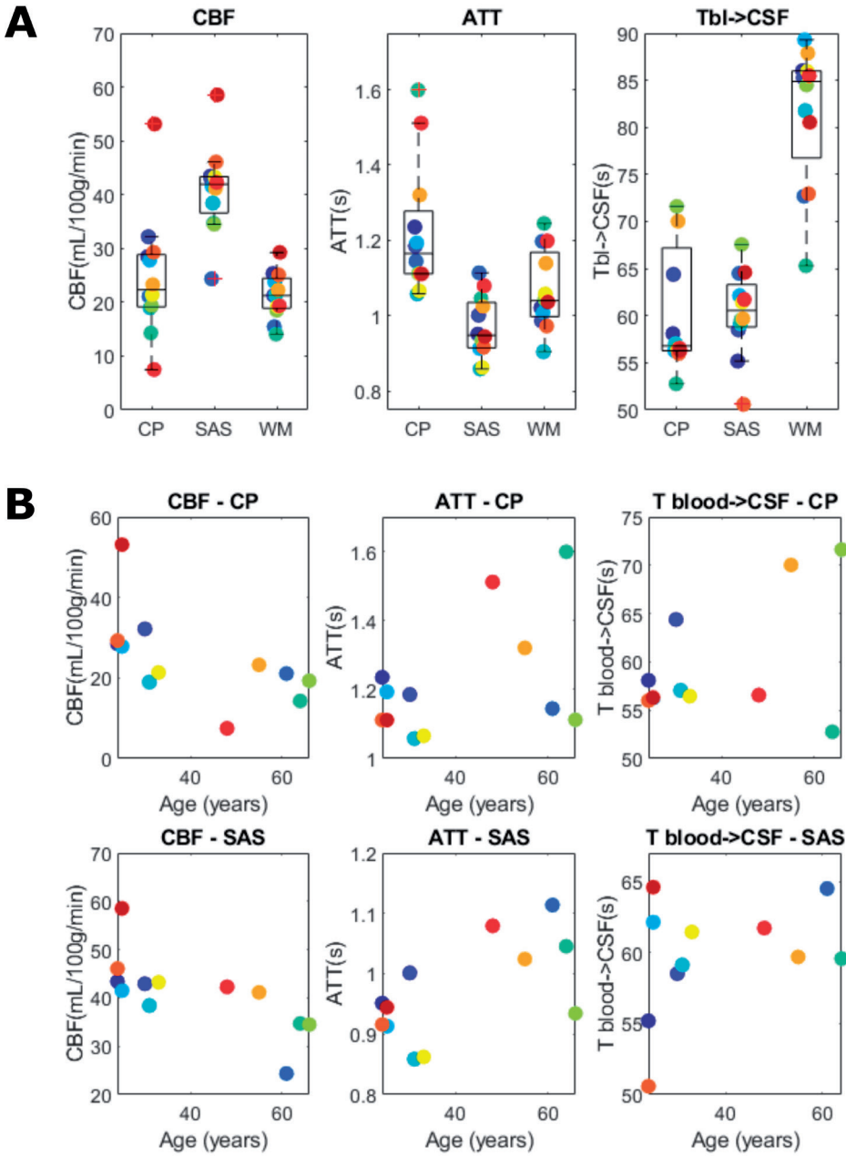
Figure 3.9. Dynamic compartmental model parameter averages per subject for (a) the choroid plexus (CP), subarachnoid space (SAS) and white matter (WM) ROIs and (b) plotted as a function of age for the CP and SAS ROIs.
