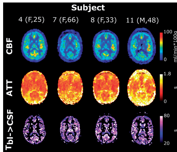
Figure 3.8. Single-slice parameter maps for four subjects with variable age and sex. T_{bl \rightarrow CSF} is shown only in the gray matter and CSF masks for easier visualization (white matter areas are particularly noisy).
