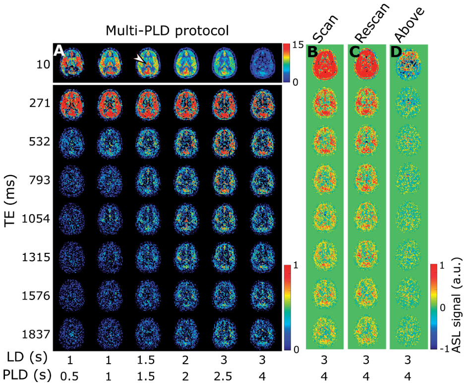
Figure 3.4. ASL signal and validation. A) ASL signal from the multi-PLD protocol for subject 1 in a single slice at all inflow time points (left to right) and echo times (top to bottom). The first echo is shown in a different scale for better visualization. In B the last column of A is repeated with the inclusion of negative signal for comparison to the validation scans. The arrowhead points to the choroid plexus (present in all images but especially visible at this time point in the perfusion image). C shows the ASL signal of the reproducibility scan (note that images are not co-registered and therefore slices may not correspond perfectly) and D shows the signal with the labeling plane above the brain.
