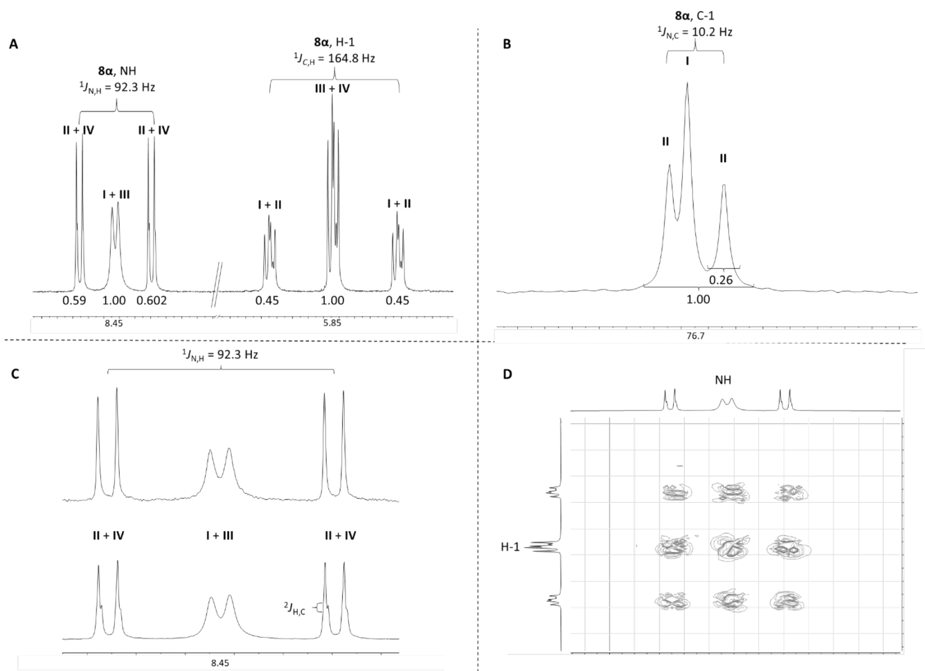
Figure 1. (A) ^1\text{H} NMR of product 8α , zoomed in onto the NH and H-1 regions. (B) ^{13}\text{C} NMR of product 8α , zoomed in onto C-1. (C) (Top) ^{13}\text{C} -decoupled ^1\text{H} NMR of product 8α , zoomed in onto the NH region and (bottom) “normal” ^1\text{H} NMR. (D) COSY of product 8α , zoomed in onto the region between H-1 and NH.
