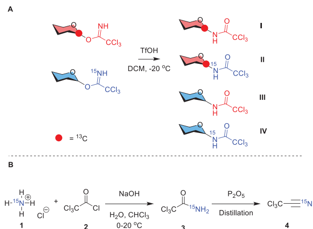
Scheme 2. (A) Starting Materials and Products of the 13 C/ 15 N Exchange Experiments and (B) Synthesis of 15 N-Labeled Trichloroacetonitrile
