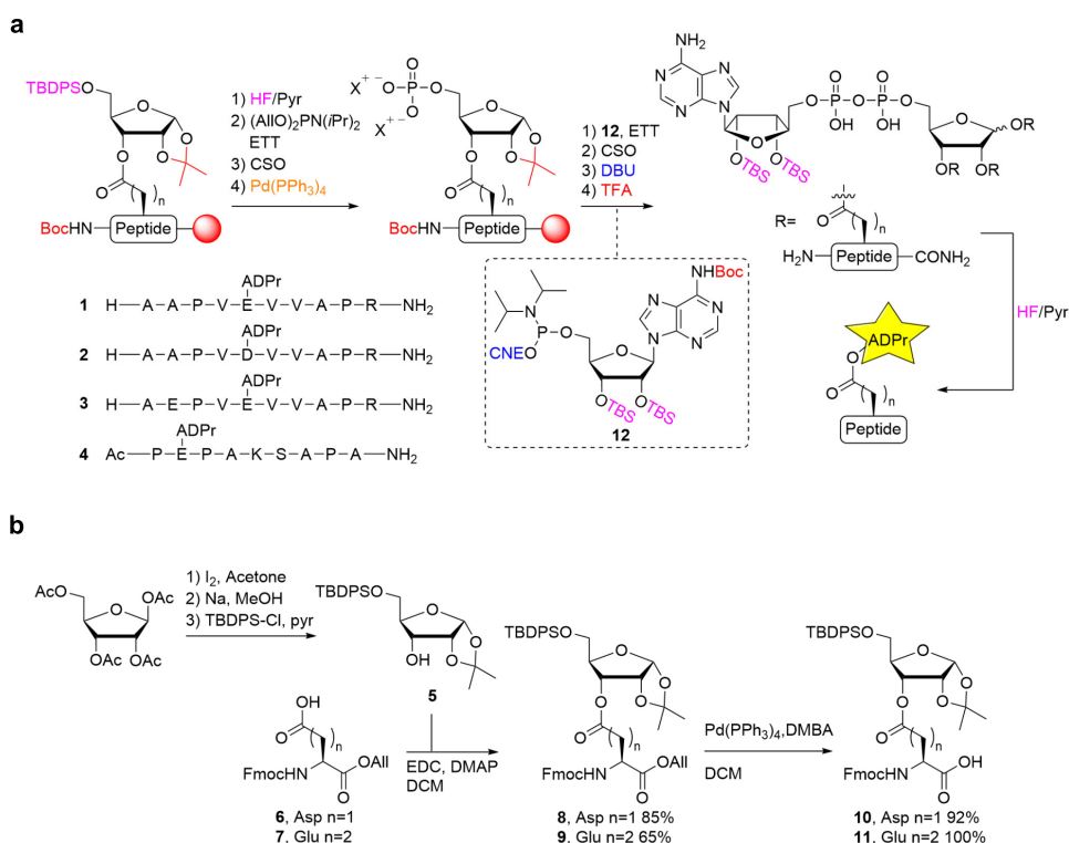
Figure 3. Total synthesis of Asp/Glu-ADP-ribosylated peptides. (a) Synthetic scheme for on-resin phosphorylation and pyrophosphorylation, resin cleavage, and tandem deprotection to generate various Asp/Glu-ADP-ribosylated peptides (compounds 1–4). Colored protecting groups indicate liability toward the respective deprotection reagent. (b) Synthetic scheme for the protected, ribosylated aspartate (compound 10) and glutamate (compound 11) building blocks that were employed in solid-phase peptide synthesis.
