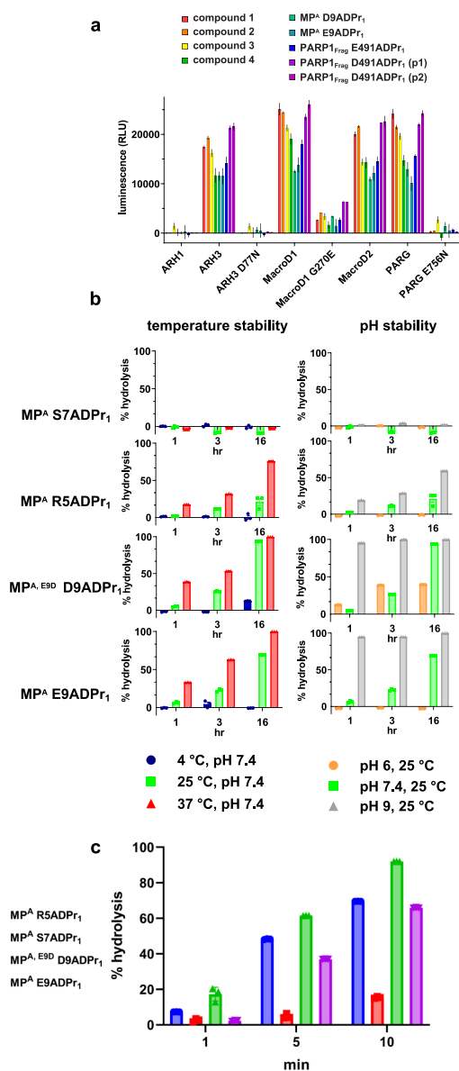
Figure 4. Enzymatic and nonenzymatic hydrolysis properties of various ADPr linkages. (a) Activity measurements for indicated wild-type and mutant ADP-ribosylhydrolase enzymes with various chemoenzymatically modified and fully synthetic Asp/Glu-ADP-ribosylated substrate peptides. (p1) and (p2) denote peak 1 and peak 2 of Figure 2a, respectively. For all measurements: n = 3 , error bars = SD. (b) Percent hydrolysis of the indicated ADPr linkage after incubation at various temperatures and pH values as measured by RP-HPLC/MS. For all measurements: n = 3 , error bars = SD. (c) Percent hydrolysis of the indicated ADPr linkage after incubation in SDS-PAGE sample preparation conditions as measured by RP-HPLC/MS. For all measurements: n = 3 , error bars = SD.
