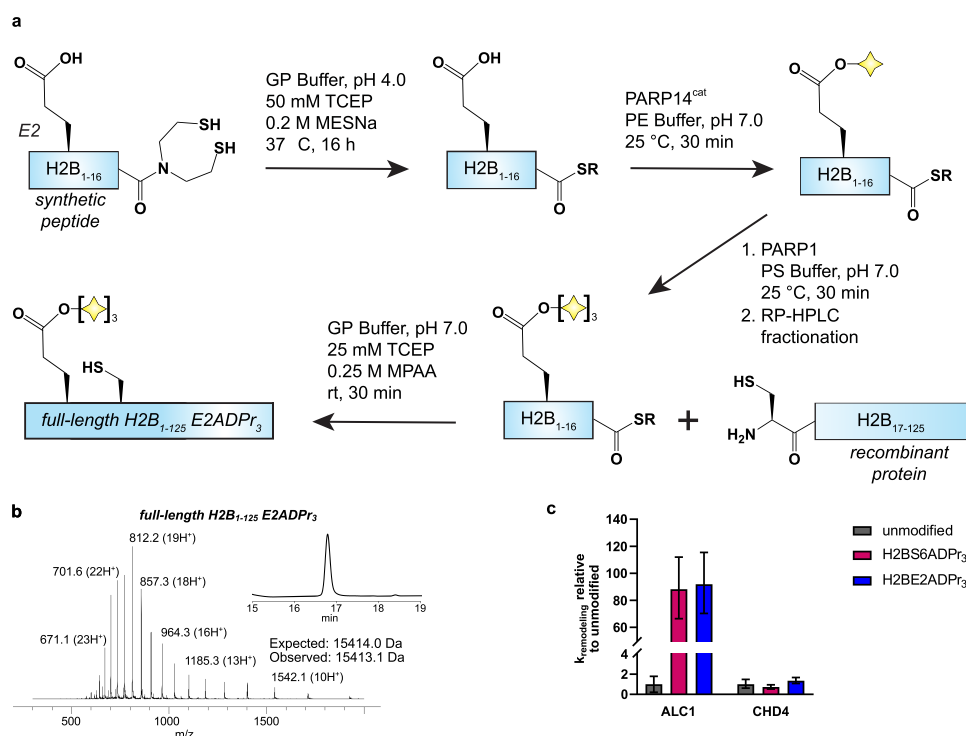
Figure 5. Semisynthetic nucleosomes bearing histone H2B E2ADPr 3 are robust substrates for the chromatin remodeler ALC1. (a) Semisynthetic scheme to prepare full-length H2B E2ADPr 3 . GP buffer = 6 M guanidine-HCl, 0.1 M sodium phosphate; SR = MES thioester. PE buffer = 50 mM Tris pH 7.0, 20 mM NaCl, 2 mM MgCl 2 , 10 mM NAD + . PS buffer = PE buffer supplemented with 10 μM PARP stimulating DNA and 2 mM TCEP. (b) Characterization of the full-length H2B E2ADPr 3 protein. Raw ESI-MS spectra and RP-HPLC chromatogram are shown. (c) Nucleosome remodeling assay time-course wherein each reaction comprises the indicated remodeler and the indicated nucleosome. “ k_{\text{remodeling}} relative to unmodified” is the rate constant of the indicated remodeling reaction relative to that of the unmodified nucleosomes: n = 3 , error bars = 95% confidence interval.
