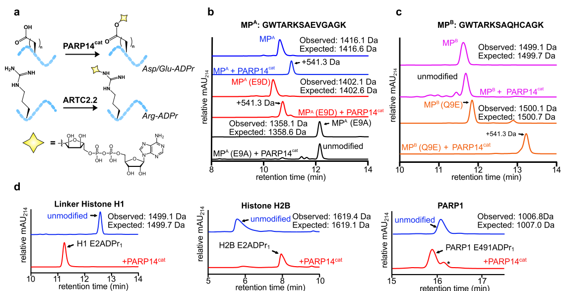
Figure 1. Chemoenzymatic generation of Asp- and Glu-ADP-ribosylated peptides. (a) Schematic depicting enzyme-catalyzed installation of mono-ADPr at Asp/Glu- and Arg-side chains on synthetic peptides via PARP14 cat and ARTC2.2, respectively. (b) RP-HPLC/MS analysis of model peptide MP A and mutant thereof pre- and postincubation with PARP14 cat . Note: mono-ADP-ribose adduct = 541.3 Da. (c) As in (b) but with model peptide MP B . (d) RP-HPLC/MS analysis of peptides containing endogenous Glu-ADPr sites pre- and postincubation with PARP14 cat . All intact ESI-MS analyses are shown in Figures S1 and S4. *unmodified peptide.
