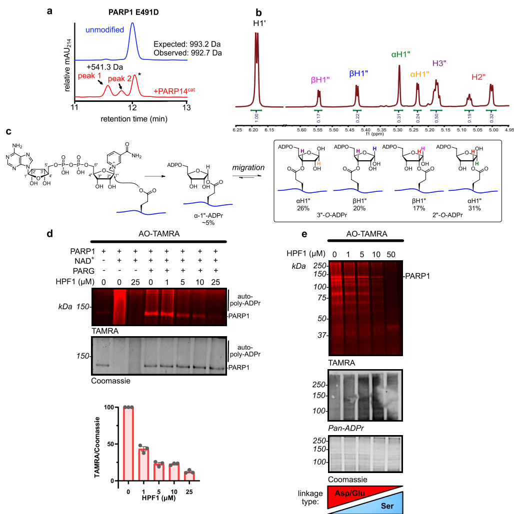
Figure 2. Structural and biochemical characterization of Asp/Glu-ADPr linkage acyl migration. (a) RP-HPLC/MS analysis of PARP1 Frag , E491D pre- and postincubation with PARP14 cat . *Unmodified peptide. (b) 1 H-NMR spectrum of PARP1 Frag E491ADPr 1 peptide. Assigned peaks are labeled with their respective protons. Color corresponds with the different isoforms found in (c). (c) Proposed mechanism for Asp/Glu-ADPr linkage migration and relative isomer abundances derived from integration of the signals as compared to the H-2 signal of the adenosine. (d) Recombinant PARP1 auto-ADPr assays in the presence of increasing HPF1 concentrations. Samples were incubated with AO-TAMRA probe and resolved by SDS-PAGE prior to analysis via in-gel fluorescence imaging or Coomassie staining (top). Poly-ADPr was converted to mono-ADPr via PARG treatment to enable quantification ( n = 3, error bars = SD) of AO-TAMRA labeling via densitometry (bottom). (e) ADPr activity in intact nuclei from HEK293T HPF1 -/- cells in the presence of increasing concentrations of recombinant HPF1. AO-TAMRA labeling and total ADPr activity are visualized via in-gel fluorescence and pan-ADPr detection reagent western blot, respectively.
