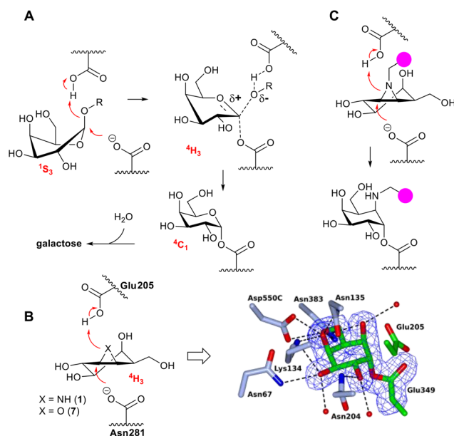
Fig. 1 (A) GALC and GLB1 are retaining \beta -galactosidases that process their substrates in a Koshland two-step double displacement mechanism, with the substrate \beta -galactoside undergoing a 1\text{S}_3-4\text{H}_3-4\text{C}_1 reaction itinerary in the first half of the catalytic cycle leading to the covalent enzyme–substrate intermediate. (B) Structure of the Cellvibrio japonicus retaining \beta -galactosidase CjGH35A , which reacts with \beta -galactose-configured cyclophellitol (7) (galactose-configured cyclophellitol aziridine reacts in the same manner 36 ). \beta -Gal-Cyclophellitol adopts a 4\text{H}_3 -configuration emulating that of the transition state of CjGH35A -mediated substrate processing. Nucleophilic opening of the epoxide by the CjGH35A Asn281 nucleophile then leads to a 4\text{C}_1 -bound enzyme–inhibitor complex which by nature of the more stable (ester as opposed to acylal that would emerge from \beta -galactoside processing) enzyme–inhibitor linkage is stable over time. (C) Substituted \beta -galactose-configured cyclophellitol aziridines as \beta -galactosidase activity-based probes, the subject of the here-presented studies (the purple bulb represents biotin or a fluorophore).
