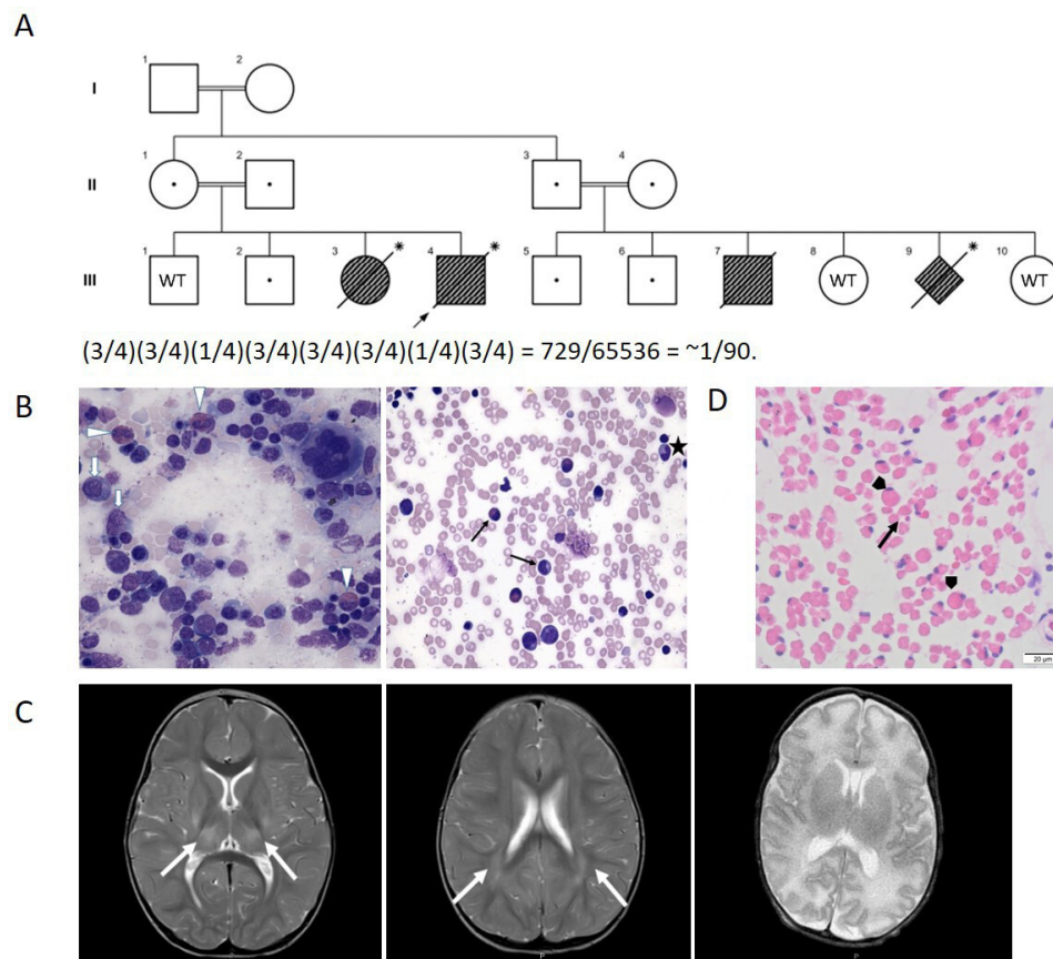
Figure 2 The sentrin-specific protease (SENP)7-related disorder. (A) A simplified pedigree of the family is shown. Note II-1 and II-2 are first cousins as well. Affected patients are marked in grey, asterisk marks the presence of the homozygous stop-gain variant p.(Gln492*) in SENP7 . For III-7 a DNA sample was not available. All healthy family members were tested and were found to be a carrier of the SENP7 variant (central dot) or wild type (WT). Co-segregation evidence was calculated based on the result in each tested subject except for the proband and the parents in both sibships. For example, the probability III-3 is homozygous mutant is 1/4, the probably III-1 and III-2 are not homozygous mutant is (3/4)^2 and so on. (B) Bone marrow aspirate showing myeloid maturation arrest. Most of the myeloid cells present are either at the promyelocytic (white arrows), myelocytic (black arrows) or metamyelocytic (star) stages of maturation. There is a notable increase of erythroid and eosinophils precursors (arrow heads). Prominent lymphocytosis is seen. (C) Left image: axial T2-weighted (T2W) image at the level of the basal ganglia. Symmetrical foci of T2 hyperintensity are noted in the lentiform and thalami bilaterally (arrows). The ventricles are within normal limits. Middle image: axial T2W image at the level of the lateral ventricles. There are confluent areas of T2 hyperintensity at the periventricular and deep white matter in the biparietal region (arrows). Right image: axial T2W at the level of the basal ganglia. Myelination is delayed. (D) A psoas muscle transverse section. Variability in size of muscle fibres, hypertrophic fibres (arrow heads) alternating with thin atrophic fibres (arrows) (H&E).
