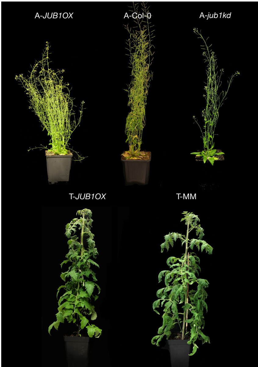
Supplementary Figure S1 Growth form of genotypes of Arabidopsis and tomato used for stem anatomical and stem P_{50} studies. A-JUB1OX (top left, 65d after sowing), A-Col-0 (top middle, 55d after sowing), A-jub1kd (top right, 55d after sowing), T-JUB1OX (bottom left, 55d after potting) and T-MM (bottom right, 55d after potting).
