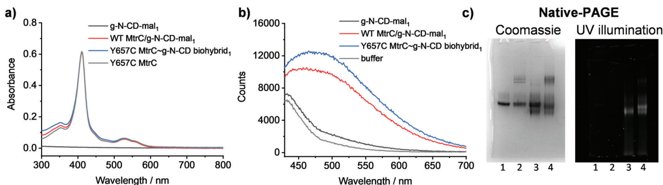
Figure 6. a) UV-vis absorption spectra and b) Fluorescence emission spectra of the strep tag column elution fractions. c) Native-PAGE images visualized by Coomassie Blue (left) and under UV illumination (right). Lanes: 1. WT MtrC, 2. Y657C MtrC, 3. Elution fraction of WT MtrC/g-N-CD-mal 1 , 4. Elution fraction of Y657C MtrC~g-N-CD biohybrid 1 . The slowest migrating bands in the Y657C MtrC samples (Figure 6c, lane 2 and 4) are MtrC dimers. Samples prepared by approach 1. pH 7.0, 20 mM MOPS, 30 mM Na 2 SO 4 , 21 °C.
