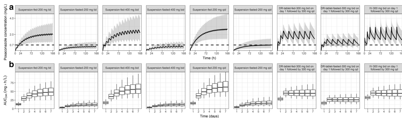
Fig. 4 Distribution of posaconazole concentration–time profiles (a) and distribution of the area under the curve per day ( AUC_{24h} ) (b) in 1000 simulated healthy volunteers receiving commonly prescribed posaconazole regimens for the oral suspension, delayed-release tablet (DR-tablet), and intravenous infusion (IV). Profiles for oral formulations were simulated under both fed and fasted conditions. In (a), the solid lines represent the median concentration, and the shaded areas
