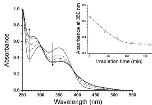
Fig. 6 UV-vis spectra measured at diluted condition after different irradiation times (0–160 min). Inset: the obtained absorbance at 350 nm was plotted as a function of irradiation time.
