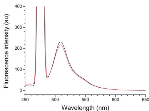
Fig. 9 Fluorescence spectra of a GFP solution ( 2 \mu\text{g mL}^{-1} ) in PBS measured before (black line) and after 30 min of UV-irradiation (red line). The GFP fluorescence did not change significantly by UV irradiation ( ca. 95% of the emission at 509 nm).
