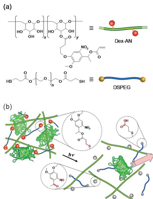
Scheme 1 Chemical structures of the components of in situ forming photodegradable hydrogel: dextran functionalized with acrylate-modified o -nitrobenzyl moieties (Dex-AN) and dithiolated poly(ethylene glycol) (DSPEG). Upon mixing, these underwent Michael addition between acrylate and thiol groups to form a light sensitive hydrogel. Upon the irradiation, the hydrogel was decomposed due to the cleavage of the photolabile moiety, which triggered the release of the protein (GFP) entrapped in the polymer network.
