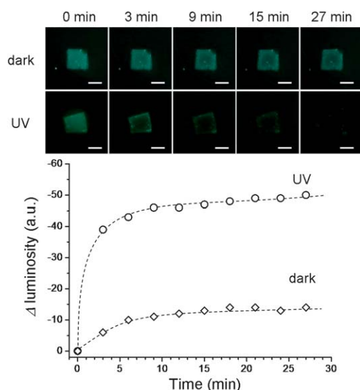
Fig. 8 Release of GFP from the gel matrices upon the irradiation with UV light. Pictures show representative states of the gel matrices for both samples kept in the dark and under UV irradiation taken with fluorescence microscope. Scale bars represent 200 \mu\text{m} . The difference of the luminosities of the gels from the original state is calculated from the pictures and plotted as a function of time.
