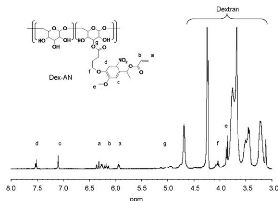
Fig. 1 1 H NMR spectrum of Dex-AN (DMSO- d 6 containing 5% D 2 O). The chemical structure shows the substitution of AN at C-3 position of glucose unit as a possible structure.
