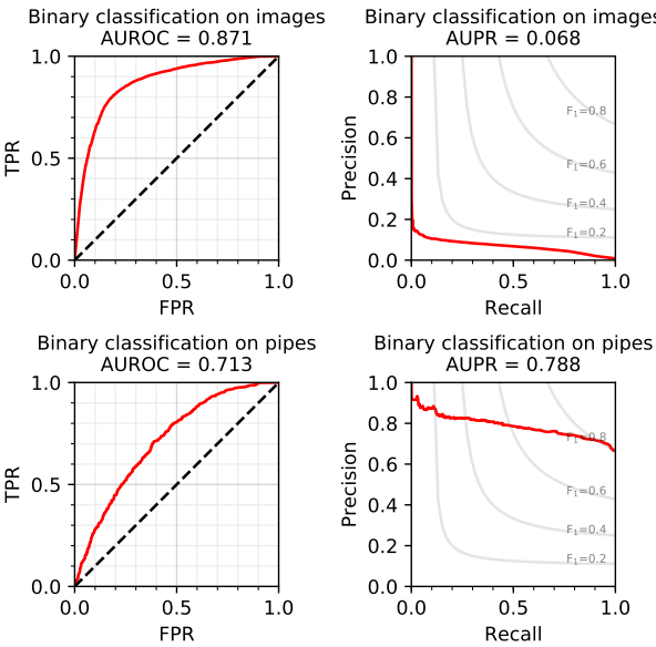
Figure 4.8: ROC and PR curves obtained when treating the problem as a binary classification problem, for image level or pipe level.
