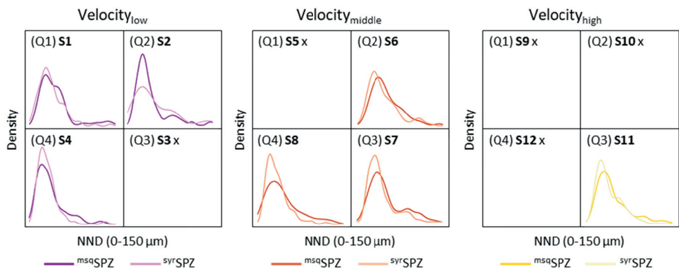
Sup. Figure S4 Relation between motility parameters and nearest neighbor distance. The nearest neighbor distance (NND) is plotted for the tracks split into 12 subsets (S1-12) based on four specific movement patterns (Q1-4, see Figure 6) and three velocity categories (1: <0.1 \mu\text{m/s} , depicted in purple; 2: 1-2 \mu\text{m/s} , depicted in orange; 3: >2 \mu\text{m/s} , depicted in yellow). The NND of the msqSPZ is depicted in the darker color and the NND of the svrSPZ is depicted in the lighter color.
