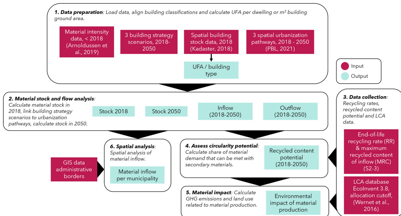
FIGURE 1 Model overview
