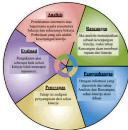
Gambar 7.4 Diagram ADDIE
