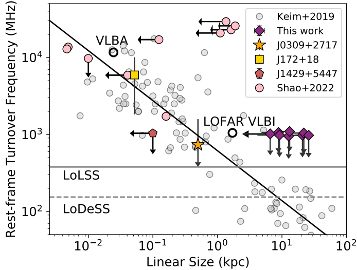
Figure 6.5: Linear sizes versus rest-frame turnover frequency for the quasars in our sample, J172+18, and the 10 high- z quasars from Shao et al. (2022). The grey points show low-redshift ( z \approx 0.1 -2) peaked spectrum sources from Keim et al. (2019), which follow a tight relation given by the black solid line (see Keim et al. 2019). Apart from J0309+2717, we have only upper limits on the linear sizes of the quasars in our sample and their turnover frequencies. Five of the quasars from Shao et al. (2022) have been observed at mas resolution with the VLBA and three of them have size measurements, which seem to follow the low- z relation. The solid and dashed grey lines show the frequencies of the LoLSS and LoDeSS survey, respectively, and the black open circles the resolution of the LOFAR VLBI and VLBA at 150 MHz and 1.6 GHz (observed frame).
