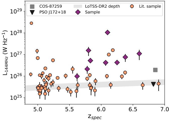
Figure 6.1: Radio luminosities at 144 MHz versus spectroscopic redshift of our selected sample and other known LOFAR detected quasars compiled by Gloudemans et al. (2021b, 2022). Our sample probes some of the brightest and highest redshift radio-loud quasars currently known at low frequencies. The heavily obscured AGN COS-87259 is currently the highest redshift radio-loud quasar known and has been detected by LOFAR (Endsley et al. 2022a, 2023). The two radio-loud quasars around z \sim 6.1 (J1427+3312 and J1429+5447) have not been included in our sample because their radio spectra have already been studied by Shao et al. (2020) and Shao et al. (2022), with J1427+3312 showing a turnover around 1.7 GHz rest-frame.
