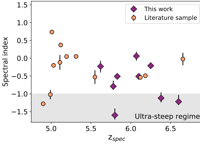
Figure 6.3: Radio spectral indices measured in this work versus spectroscopic redshift. The spectral indices of known quasars compiled by Gloudemans et al. (2021b, 2022) that are detected by LOFAR and either FIRST or VLASS are plotted for comparison. The sources from Fig. 6.1 without radio spectral index measurements are excluded. Our sample covers a wide range of spectral indices and contains 3 sources that could be classified as ultra-steep spectrum sources ( \alpha < -1.0 ).
