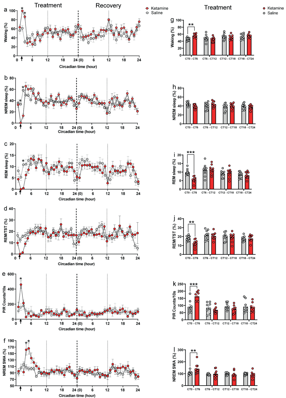
Figure 2. Vigilant stages, locomotor activity and slow-wave activity in NREM sleep after ketamine and saline treatment. a – f. Time course of waking, NREM sleep, REM sleep, REM sleep/ Total sleep time, locomotor activity and slow-wave activity (SWA) in NREM
