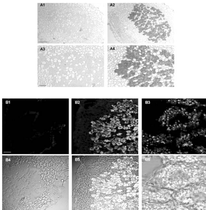
Figure 2. Comparison of results obtained with the same primary antibody (MnSOD) and either AP-detection (A) or fluorescent detection (B). Immunolocalisation of MnSOD in Lotus japonicus nodules. Images represent longitudinal sections of 13 days post inoculation (dpi) nodules. Alkaline phosphatase-conjugated (A) and alexa488-conjugated (B) anti-rabbit immunoglobulin Gs were used as secondary antibodies. A3 and A4 are magnifications of A1 and A2, respectively. B1, B2, and B3, are the confocal microscope images showing the signal in the infected cells of the central tissue (background subtracted). B4, B5, and B6, are overlays of B1, B2, and B3, and the corresponding transmitted light images. B3 and B6 are a high magnification of the central tissue. No signal was observed in the controls (A1, A3, B1, B4). Bars = 50 µm (A1 and A2), 30 µm (B1, B2, B4, and B5), 20 µm (A3 and A4), and 3 µm (B3 and B6). See colour plate 3 (G) for a colour version of B1-B6.
