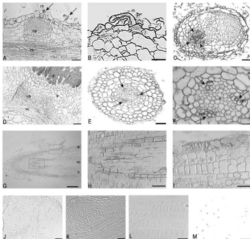
Figure 1. Localisation of LjSBP1 in root tips and roots. Immunolocalisation of the selenium binding protein (SBP) of Lotus japonicus on roots, nodules and root tips. Detection was performed with alkaline phosphatase conjugated secondary antibodies. The embedding of the root tissue in BMM resulted in sections of high cellular resolution, enabling the detection of SBP in cellular structures that are otherwise difficult to preserve in detail, like root hairs (A), infection threads (B), and the phloem of the vascular cylinder (C). Furthermore, signal was detected in the vascular bundles and the infected cells of the central tissue in mature nodules (D). H and I are differential interference contrast microscopy pictures of the marked regions in picture G. Signal was observed in the cells of the epidermis and the outer cortex of the root tip (I) as well as on the vasculature (H). Transverse sections of that area allowed the identification of the protophloem cells of the stele as the cells with high expression levels of the protein (E and F). J-M sections incubated with pre-immune serum. A to D, G, J, K, bars=50µm. E, M, bars=25µm.
