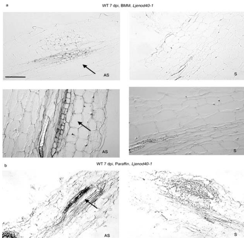
Figure 3. The weak signals obtained for RNA localisation of Ljenod40-1 transcripts are compared to signals obtained on paraffin sections. Ljenod40-1 localises in the pericycle cells at the base of dividing cortical cells. The signal obtained on BMM embedded tissue (a) is much lower, but the cellular resolution/tissue preservation better compared to the paraffin embedded tissue (b). AS, sections probed with antisense Ljenod40-1 transcript. S, sections probed with sense Ljenod40-1 transcript, as negative control. Arrows indicate signal. Detection was performed with alkaline phosphatase-conjugated anti-DIG primary antibody. Bar = 100 \mu m.
