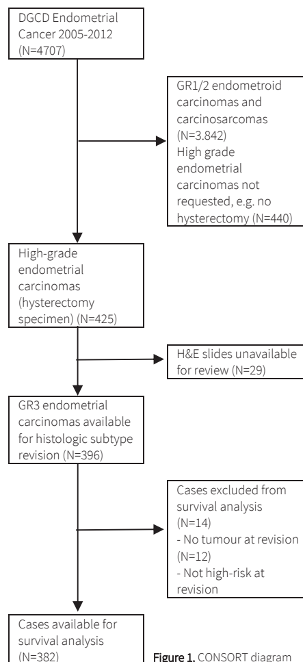
Figure 1. CONSORT diagram
