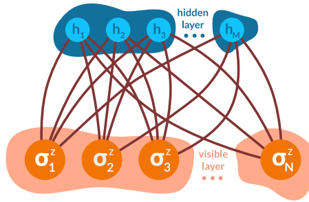
Figure 4.1: Illustration of a restricted Boltzmann machine (RBM) neural network.
