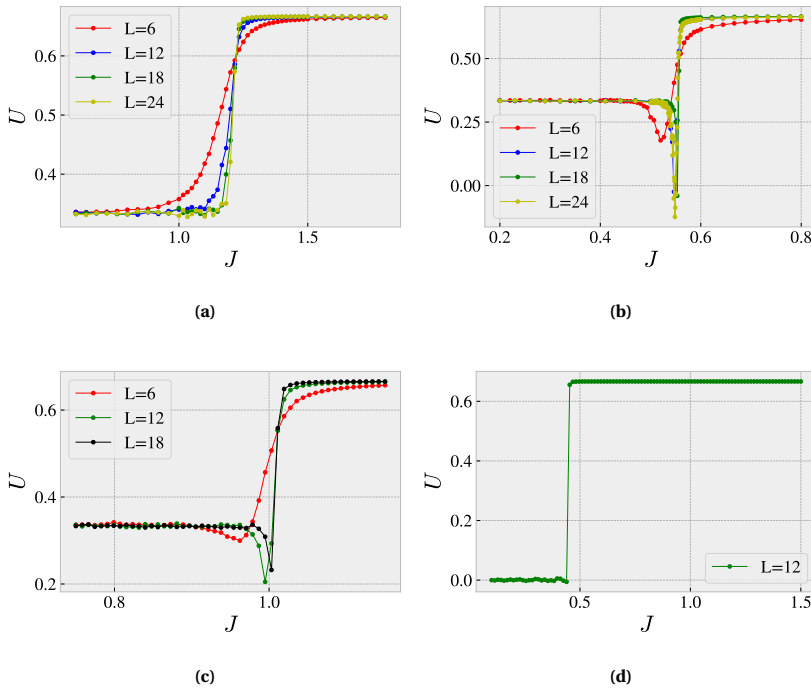
Figure 3.15: Examples of the Binder ratio as function of system size: (a) : A typical example of a second order transition from confining to Higgs for O(2)/Z_2 at K=0 , (b) : An example of a first order transition for O(2)/Z_2 at value of K in the range of first order - "Huse-Leibler" line emanating from the tricritical point (c) : An example of the Binder ratio for a weak first order transition, showing its behavior for O(2) \times O(2)/Z_2 for K=0 as function of J . (d) An example of the Binder ratio for Z_2 \times Z_2 \times Z_2/Z_2 along K=0 with a clear indication of a second order phase transition.
