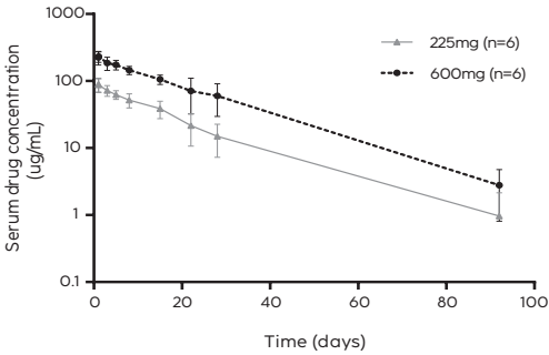
FIGURE 4 SEMI-LOG MEAN SERUM CONCENTRATION VERSUS TIME PROFILES OF ENSOVIBEP FOLLOWING 225- AND 600-MG ADMINISTRATION.
