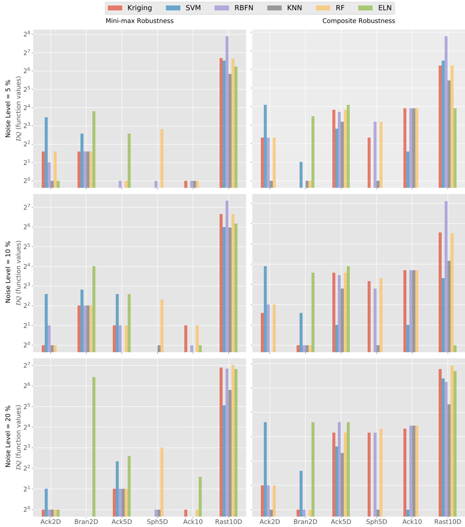
Figure 3.10: The difference in the quality DQ of the robust solutions (obtained from surrogate modeling), for all thirty six test scenarios. Note that the quality in this context is based on the objective function values, measured according to Eq. (3.12). Furthermore, the number of independent runs in this context are set to be 100.
