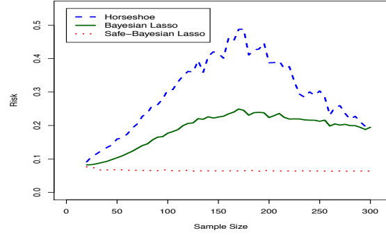
Figure 3: Simulated squared error risk (test error) with respect to P as function of sample size for the wrong-model experiments of Section 5.1 using the posterior predictive distribution of the standard Bayesian lasso (green, solid), the Safe-Bayesian lasso (red, dotted), both with standard improper priors, and the Horseshoe (blue, dashed); and 201 Fourier basis functions.
