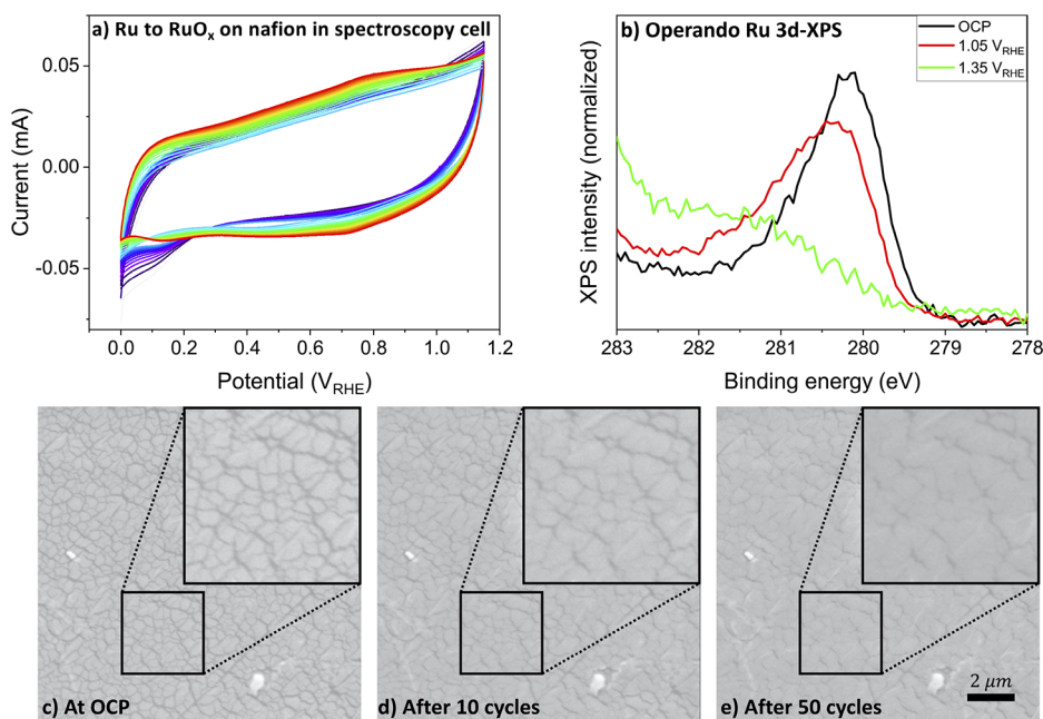
Figure 3. Electrochemical oxidation of sputter deposited ruthenium films. (a) Cyclic voltammogram of metallic ruthenium recorded in the spectroscopy cell using 0.1 M H 2 SO 4 as electrolyte at 50 mV/s. The initial cycles are purple and later are red in color. (b) Operando Ru 3d XPS of a metallic ruthenium film sandwiched between graphene and Nafion membrane. (c–e) Operando electrochemical SEM micrographs of a ruthenium film covered with graphene at OCP, after 10 cycles, and after 50 cycles of anodic polarization.
