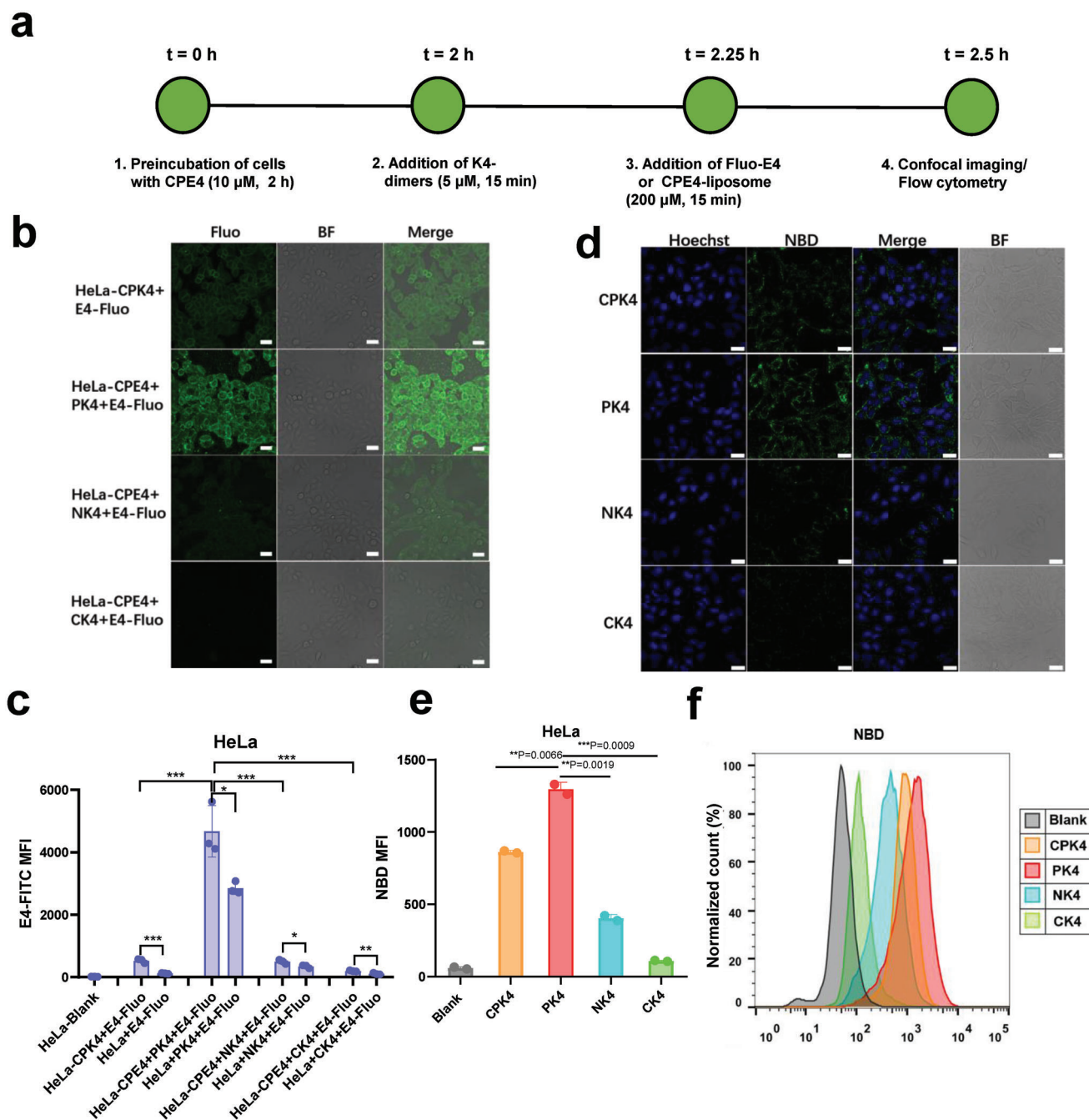
Figure 5. Cell labeling and cell uptake studies. a) Schematic representation of the cell labeling and cell uptake experiments of K4 dimer with cells. b) Confocal images of cell membrane labeling between K4 monomer/dimers and Fluo-E4. Green: fluorescein-E4; BF: bright field; scale bar is 30 \mu m. c) Quantification of cell membrane labeling efficiency by flow cytometry measurements. d) Confocal images of K4 monomer and dimers with fluorescent NBD-PE labeled CPE4-liposomes. e, f) Quantification of the liposome-NBD intensity of K4 monomer and dimers with cells. Green: PE-NBD; blue: Hoechst 33 342. BF: bright field; scale bar is 30 \mu m. In (d–f), CPK4: CPK4-cell+CPE4-liposome-NBD; PK4: CPE4-cell+PK4+CPE4-liposome-NBD; NK4: CPE4-cell+NK4+CPE4-liposome-NBD; CK4: CPE4-cell+CK4+CPE4-liposome-NBD. Unpaired student t -test was used to determine the significance of data comparisons (**** P < 0.0001; *** P < 0.001; ** P < 0.01; * P < 0.05). In all panels, error bars represent mean \pm s.d. ( n = 3).
