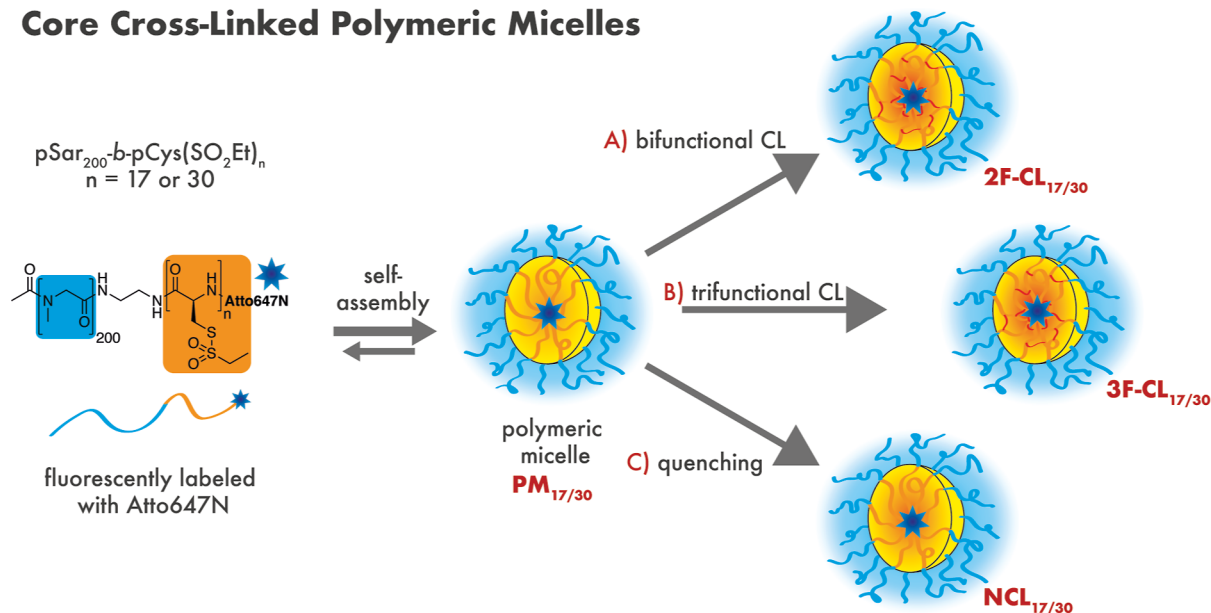
Scheme 1. Preparation of CCPMs from pSar- b -pCys(SO 2 Et) n with n = 17 or 30 (PM 17/30 ) and Thiol-Reagents of Varying Functionality
