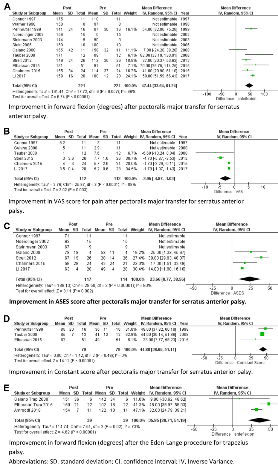
Figure 2 Forest plots. (A) Improvement in forward flexion (degrees) after pectoralis major transfer for serratus anterior palsy. (B) Improvement in VAS score for pain after pectoralis major transfer for serratus anterior palsy. (C) Improvement in ASES score after pectoralis major transfer for serratus anterior palsy. (D) Improvement in Constant score after pectoralis major transfer for serratus anterior palsy. (E) Improvement in forward flexion (degrees) after the Eden-Lange procedure for trapezius palsy. SD, standard deviation; IV, inverse variance; CI, confidence interval.
