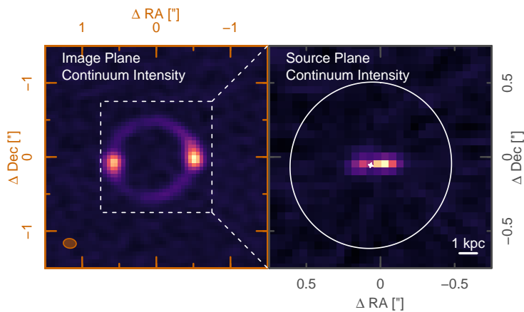
Figure 2.5: Source plane reconstruction of dust continuum emission from the ‘high’ spatial resolution \text{CH}^+(1-0) data set using LLENSTOOL. The left panel displays the observed image plane dust continuum intensity with the beam ( 0.17'' \times 0.13'' ) shown in the lower left by the shaded orange ellipse. The right panel is a zoom in of the white dashed region in the left panel, displaying the source plane reconstruction of the dust continuum. The lens caustics are indicated by the solid white lines and a physical scale of 1kpc is given in the lower right corner. A single compact and elongated source is revealed directly to the West of the inner caustic. The weak eastern feature is an artifact of beam smearing over the outer caustic in the image plane.
