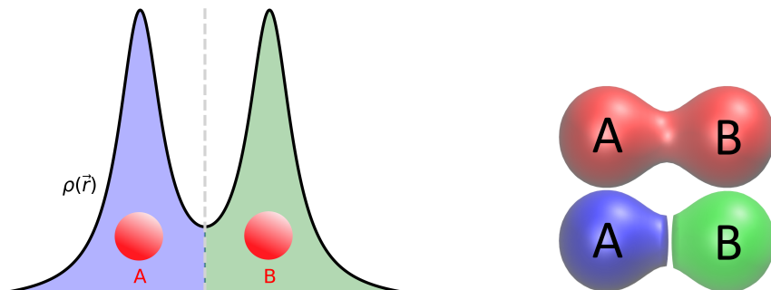
(a) One-dimensional cut through the electronic charge density \rho(\vec{r}) of an O_2 molecule. The nuclei of atom A and B are indicated by red circles, while \rho(\vec{r}) is shown on the y-axis. The surface of zero flux marked by the gray dashed line.
