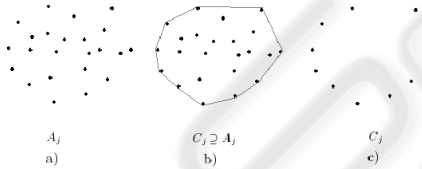
Figure 3: a) The representation of an individual A_j as a collection of points, b) an individual A_j and its convex hull C_j , c) convex boundary points C_j .
