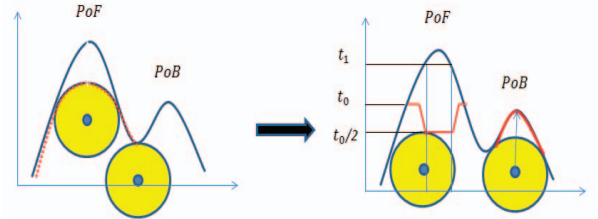
Fig. 2. Process of constructing dam in a 2D landscape. Ball path depicted as dotted line and full line respectively, in which the dotted line describes the way that original ball rolls under the image shape and full line shows the constrained path the ball can roll only according to the dam. Peak value of foreground and peak value of background are assumed as PoF and PoB respectively.
