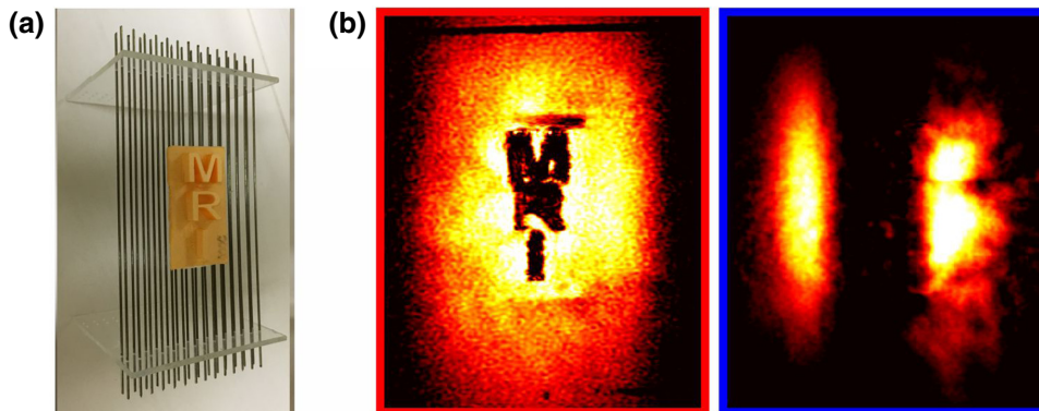
FIG. 3. (a) Photograph of the experimental setup: three-dimensional “MRI” word made from Styrofoam material is placed on top of the metasurface in the center. (b) Measured image intensities acquired with the metasurface tuned close to the first (left) and second (right) eigenmodes.
