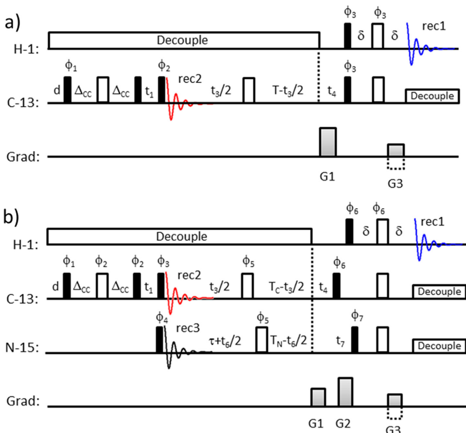
Fig. 31. PANACEA pulse sequences for a) two and b) three receivers; all pulses are applied with phase 'x', unless indicated otherwise; phase cycling (a): \phi_1 = x, -x ; \phi_2 = x, x, -x, -x ; \phi_3 = y, y, -y, -y ; rec1 = rec2 = x, -x, -x, x ; phase cycling (b): \phi_1 = 4(x, -x) 4(-x, x) ; \phi_2 = x ; \phi_3 = 2x, 2(-x) ; \phi_5 = x ; \phi_6 = \phi_7 = y, y, -y, -y ; \phi_4 = rec(all) x, -x, -x, x, -x, x, -x ; delays: \Delta_{cc} = 0.25/J(^{13}C-^{13}C) , T_c = t_2 - t_4 , where t_2 is the acquisition time for the ^{13}C receiver; T_N = t_2 - t_7 where t_7 is the ^nJ(^{15}N-^1H) evolution delay; gradients pulses, (G/cm, ms) (a): G1(40, 1) and G2(10, 1); (b): G1(20, 1), G2(20.5, 1) and G3(5, 1). Adapted from Ref. [110] with permission.
