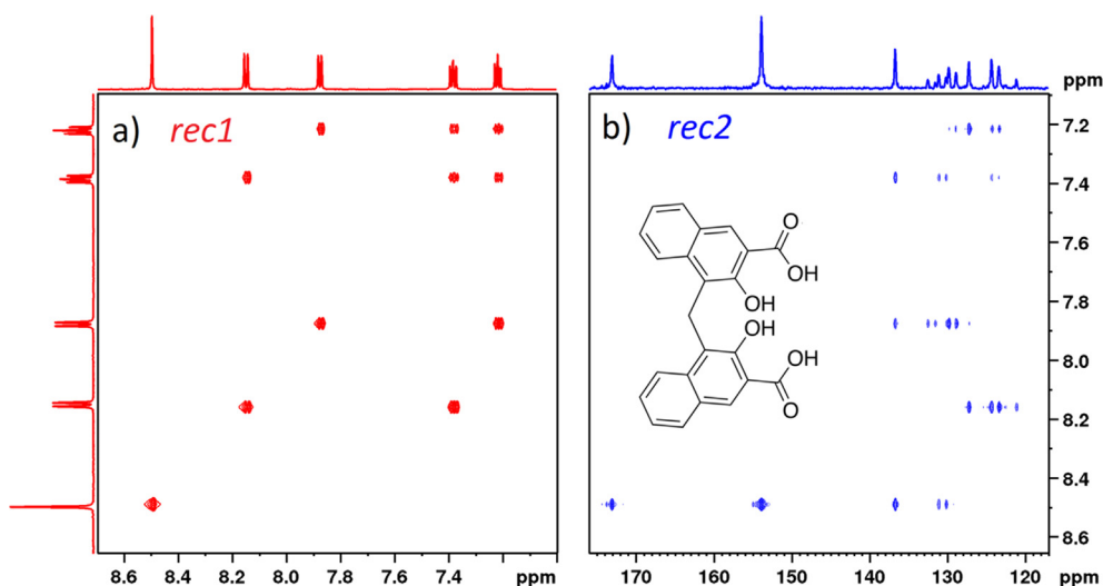
Fig. 16. Spectra of pamoic acid in \text{DMSO-}d_6 recorded with the pulse scheme of Fig. 15c on a 500 MHz ( ^1\text{H} ) Bruker Avance III HD system equipped with two receivers; a) the ^1\text{H} - ^1\text{H} COSY spectrum acquired in ^1\text{H} receiver and (b) the ^1\text{H} - ^{13}\text{C} COSY spectrum (akin to ^{13}\text{C} HMBC) acquired with ^1\text{J}(\text{H},^{13}\text{C}) suppression in the F_1 domain by the second ( ^{13}\text{C} ) receiver [105].
