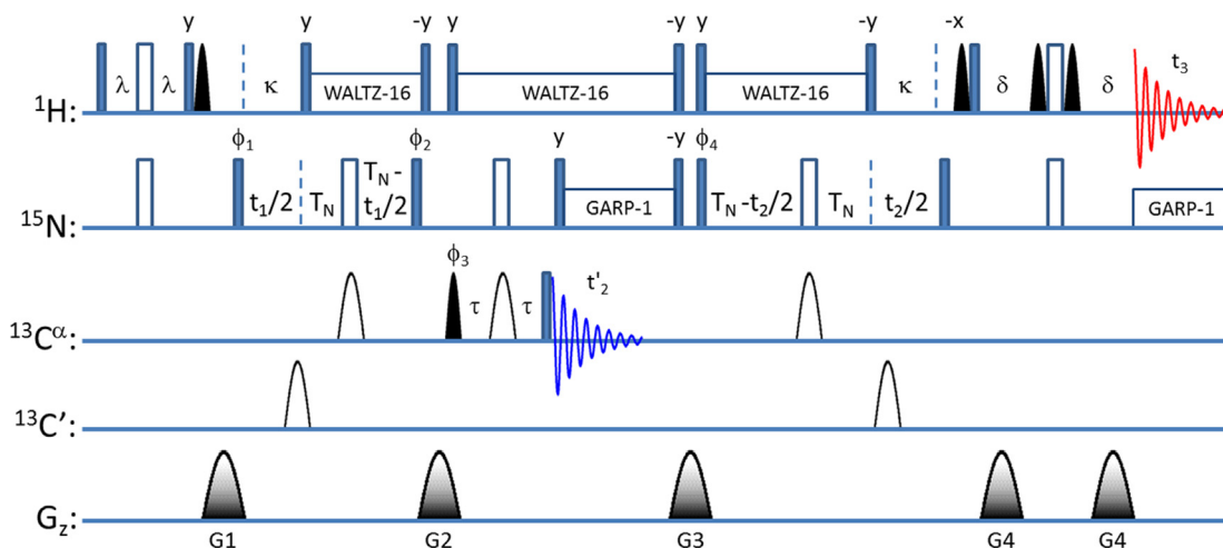
Fig. 42. The 2D (H)NCA/3D HNN pulse scheme [141]. Delays: \lambda = 2.7 ms, \kappa = 5.4 ms, \delta = 2.7 ms, T_N = 15 ms, \tau = 12 –16 ms (to be optimized), phase cycling: \phi_1 = x, x, -x, -x , \phi_2 = \phi_3 = x, -x, 4x, 4(-x) , \text{Rec}(^1\text{H}) = x, x, -x, -x, -x, -x, x, x , \text{Rec}(^{13}\text{C}) = x, x, -x, -x ; States-TPPI scheme applied to \phi_1 and \phi_4 ; gradients (1 ms, G/cm): G1 = G2 = G3 = 16, G4 = 42.
