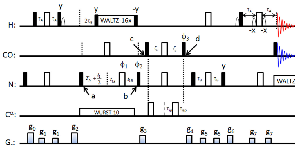
Fig. 43. Pulse scheme for a parallel ^{15}\text{N} HSQC experiment with simultaneous detection of ^1\text{H} and ^{13}\text{CO} FIDs. Delays: \tau_A = 2.5 ms, \tau_B = 2.75 ms, T_N \approx 15 ms (adjusted to achieve similar sensitivity for ^1\text{H} and ^{13}\text{CO} ), \zeta = 12.4 ms; if T_N \geq t_1/2 then t_{1A} = 0 and t_{1B} = T_N - t_1/2 , otherwise t_{1A} = t_1/2 - T_N and t_{1B} = T_N ( ^{13}\text{CO} 180° pulse duration). Phase cycling: \phi_1 = x, y, -x, -y ; \text{Rec}(^1\text{H}) = \text{Rec}(^{13}\text{C}) = x, -x ; States-TPPI applied to \phi_2 ; the IPAP scheme is implemented by setting \phi_3 = y , \tau_{ip} = \zeta and \tau_{ap} = 0 for the IP component and \phi_3 = -x , \tau_{ip} = \zeta - \tau_{ap} and \tau_{ap} = 4.86 ms for the AP component. A small angle phase shift is applied to the ^{13}\text{CO} 180° pulse between points c and d compensates for the differences in power used for this pulse and the flanking 90° pulses. Gradient pulses ( \text{G}/\text{cm} , ms): g_0 = (10, 0.5) , g_1 = (5, 0.5) , g_2 = (15, 1) , g_3 = (11, 1) , g_4 = (7, 0.8) , g_5 = (-3, 0.3) , g_6 = (5, 0.6) , g_7 = (24, 0.4) . Reproduced from Ref. [107] with permission.
