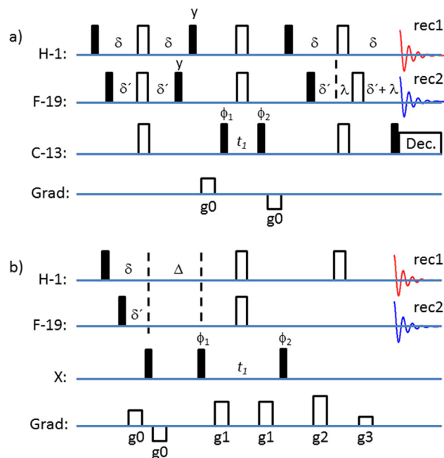
Fig. 18. a) ^1\text{H}/^{19}\text{F} - ^{13}\text{C} PANSY HSQC sequence; b) ^1\text{H}/^{19}\text{F} -X PANSY HMBC sequence; delays: \delta = 0.5/J(^1\text{H} - ^{13}\text{C}) , \delta' = 0.5/J(^{19}\text{F} - ^{13}\text{C}) , \Delta = 0.5/J(^1\text{H} -X), the \lambda delay is adjusted to ensure simultaneous refocusing of the ^1\text{H} and ^{19}\text{F} magnetization; all pulses were applied with phase 'x', unless indicated otherwise, \phi_1 = x, -x , \phi_2 = x, x, -x, -x ; \text{rec1} = \text{rec2} = x, -x, -x, x ; gradients (G/cm, ms): g_0 = (33.0, 1) , g_1 = (20, 1) , 2 g_1/(g_2 + g_3) = \gamma\text{F}/\gamma\text{X} , 2 g_1/(g_2 - g_3) = \gamma\text{H}/\gamma\text{X} ; the amplitudes of the g_1 gradient pulses were inverted every second scan for echo/anti-echo data in F_1 .
