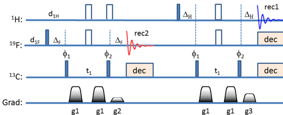
Fig. 29. The interleaved ^{19}\text{F} - ^{13}\text{C} (left) and ^1\text{H} - ^{13}\text{C} (right) HMQC experiment; delays: \Delta_F = 0.5/J(^{19}\text{F} - ^{13}\text{C}) , \Delta_H = 0.5/J(^1\text{H} - ^{13}\text{C}) , all pulses were applied with phase 'x', unless indicated otherwise, \phi_1 = x, -x , \phi_2 = x, x, -x, -x ; \text{rec1} = \text{rec2} = x, -x, -x, x ; gradient pulses (G/cm, ms): g1 = (21.4, 1) , g2 = (10.75, 1) , g3 = (11.44, 1) ; the amplitude of the g1 gradient pulses was inverted every second scan for echo/anti-echo data in F_1 ; for further experimental details see Ref. [38].
