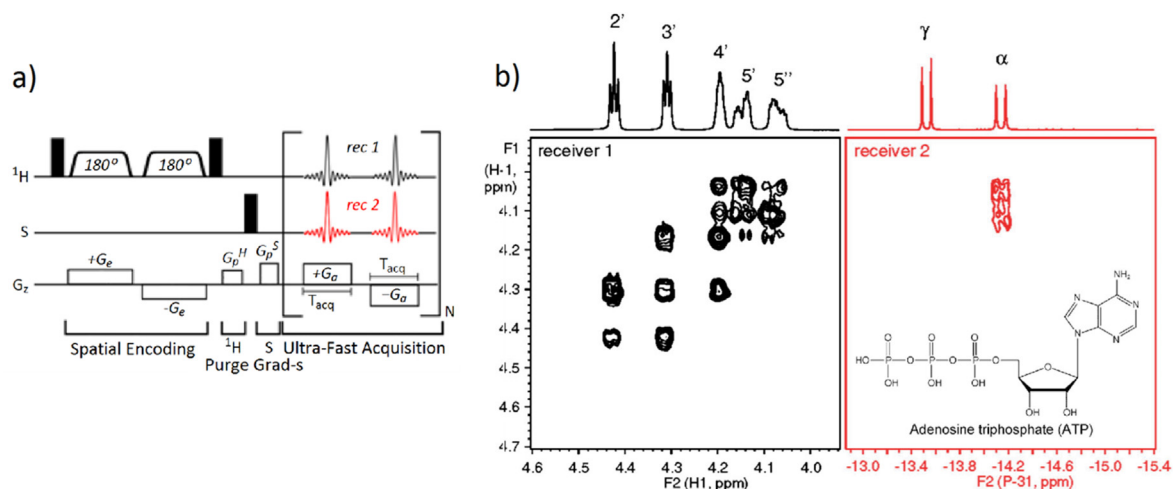
Fig. 20. a) The PUFY-COSY pulse sequence for simultaneous acquisition of ^1\text{H} - ^1\text{H} COSY and ^1\text{H} -X COSY in a single scan. b) ^1\text{H} - ^31\text{P} PUFY-COSY spectra recorded using the pulse sequence in panel (a) and S = ^31\text{P} . The ^1\text{H} - ^1\text{H} correlations detected in receiver 1 are shown in black while the ^1\text{H} - ^31\text{P} spectrum acquired in receiver 2 is shown in red. Independently recorded 1D spectra are shown above the 2D spectra; G_e = \pm 10 G/cm, G_a = \pm 9.6 G/cm; T_e = 30 ms, T_{acq} = 90 \mu\text{s} and N = 125 . Reproduced from Ref. [108] with permission.
