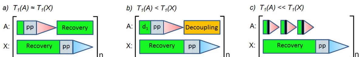
Fig. 4. Schematics of interleaved experiments. a) The FID of A-nuclei is recorded during the recovery period of X-nuclei and vice versa, where the nuclear species have comparable relaxation times and no decoupling is feasible. b) The same as in (a) except that the T_1 relaxation time of A-nuclei is significantly shorter than that of X-nuclei. The recovery period is determined by the more slowly relaxing X-nuclei, enabling decoupling of A-nuclei. c) Relaxation of A-nuclei is very fast as compared to that of X-nuclei, allowing recording of several FID-s of A-nuclei during the recovery period of X-nuclei. Decoupling of A-nuclei is possible, but may not always be needed, e.g., for quadrupolar nuclei due to self-decoupling arising from rapid relaxation.
