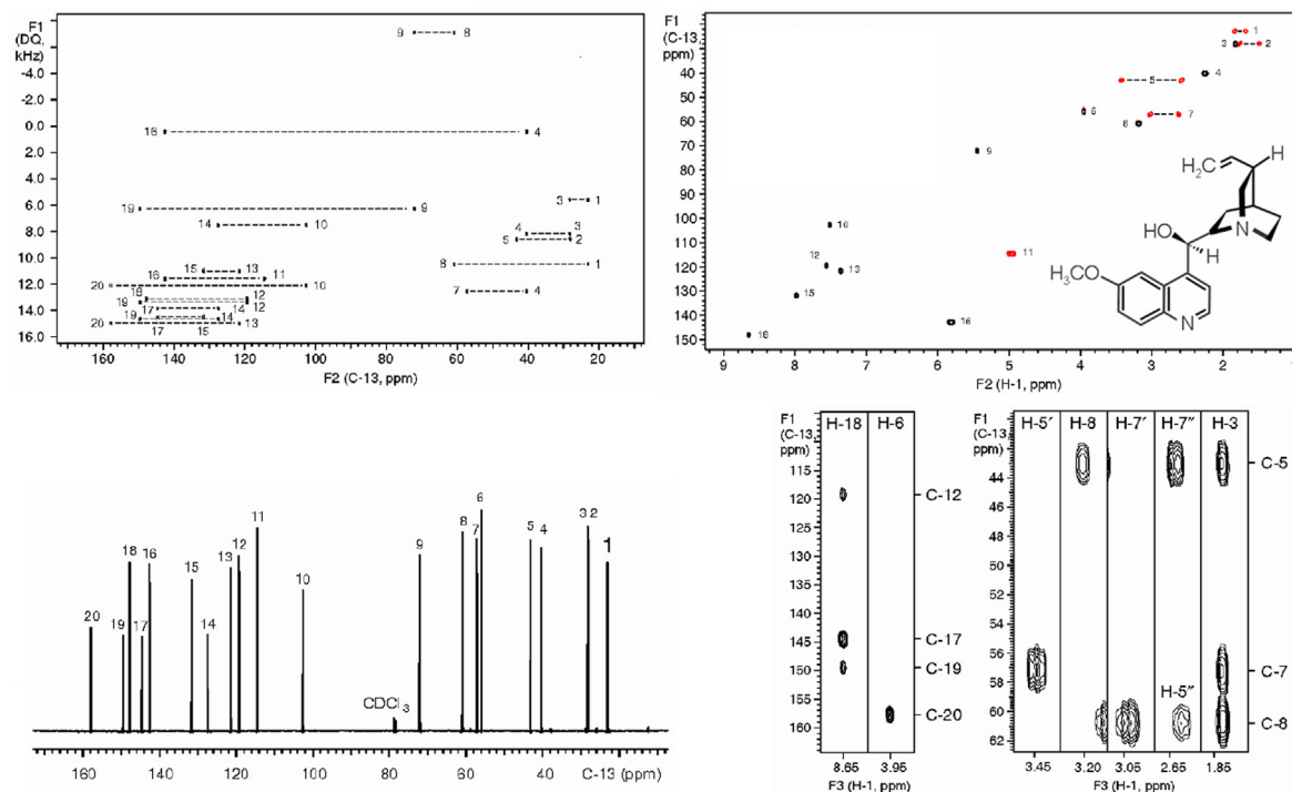
Fig. 33. PANACEA spectra of quinine in CDCl 3 recorded on a 600 MHz ( 1 H) Varian direct drive NMR system equipped with a triple resonance HCN room temperature probe; a) 2D 13 C- 13 C INADEQUATE spectrum, b) multiplicity edited 2D 13 C HSQC spectrum, c) 1D 13 C spectrum and d) strip plot of long-range correlations from the 3D 13 C J-HMBC spectrum. Experiment time was 12 h. Reproduced from Ref. [110] with permission.
