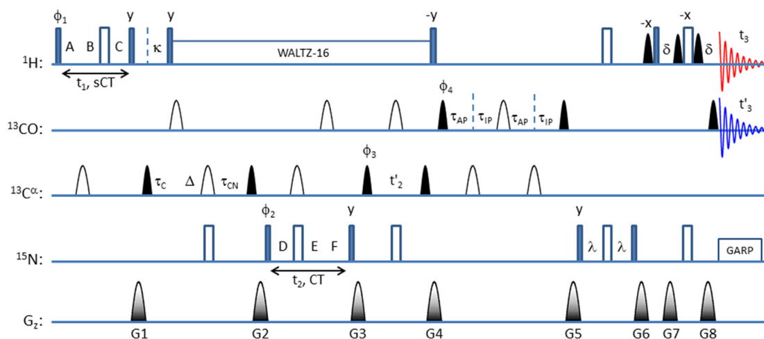
Fig. 47. 3D-HA(CA)NH / 3D-HACACO pulse scheme with parallel acquisition of ^1\text{H} and ^{13}\text{CO} nuclei. Phase cycling: \phi_1 = x, -x ; \phi_2 = \phi_3 = 2(x), 2(-x) and \phi_{\text{rec}} = x, 2(-x), x ; all other pulses are applied with phase 'x' unless indicated otherwise. States-TPPI applied to phases \phi_1 and \phi_2/\phi_3 along with phase of the corresponding receivers, \phi_{\text{rec}} . The ^{13}\text{C} carrier frequency is initially set at 54 ppm and after gradient pulse G4 is switched to 176 ppm. Gradient pulses (G/cm, 1 ms): G1 = 25, G2 = G3 = G4 = 15, G5 = G6 = 40 and G7 = G8 = 30. Delays: \kappa = 2.2 ms, \tau_C = 3.5 ms (to be optimized), \tau_{\text{CN}} = 12.5 ms, T_N = 14 ms, \lambda = \delta = 2.7 ms, and \Delta = \tau_{\text{CN}} - \tau_C ; A, B and C are semi-constant t_1 -evolution ( ^1\text{H}\alpha ) delays, D, E and F are constant time t_2 evolution ( ^{15}\text{N} ) delays. The IPAP scheme is employed for recording 3D-HACACO data set by setting \phi_4 = y , \tau_{\text{IP}} = 4.5 ms, \tau_{\text{AP}} = 0 ms for the IP component and \phi_4 = -x , \tau_{\text{AP}} = \tau_{\text{IP}} = 2.25 ms for the AP component.
