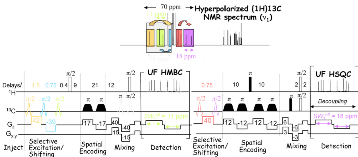
Fig. 11. Interleaved ultra-fast 2D C-H HMBC/HSQC pulse scheme (UF NOAH-2 BS supersequence) ; \delta = 0.4 ms, \Delta_1 = 9 ms, \Delta_2 = 12 ms, \tau = 0.4 ms, dwell time, dw = 2 \mu\text{s} . Reproduced from Ref. [88] with permission.
