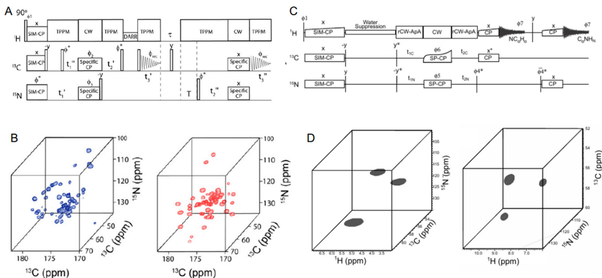
Fig. 55. Use of bi-directional polarization transfer to combine complementary 3D experiments. (A) Pulse sequence and (B) spectra for sequentially acquired 3D NCACX and 3D CANCO experiments on a sample of uniformly ^{13}\text{C} and ^{15}\text{N} labelled ubiquitin. (C) Pulse sequence and (D) spectra for sequentially acquired NCAHA and CANH spectra for a sample of ^{13}\text{C} and ^{15}\text{N} labelled MLF. (A–B) adapted from Ref. [189] with permission. (C–D) adapted from Ref. [174] with permission.
