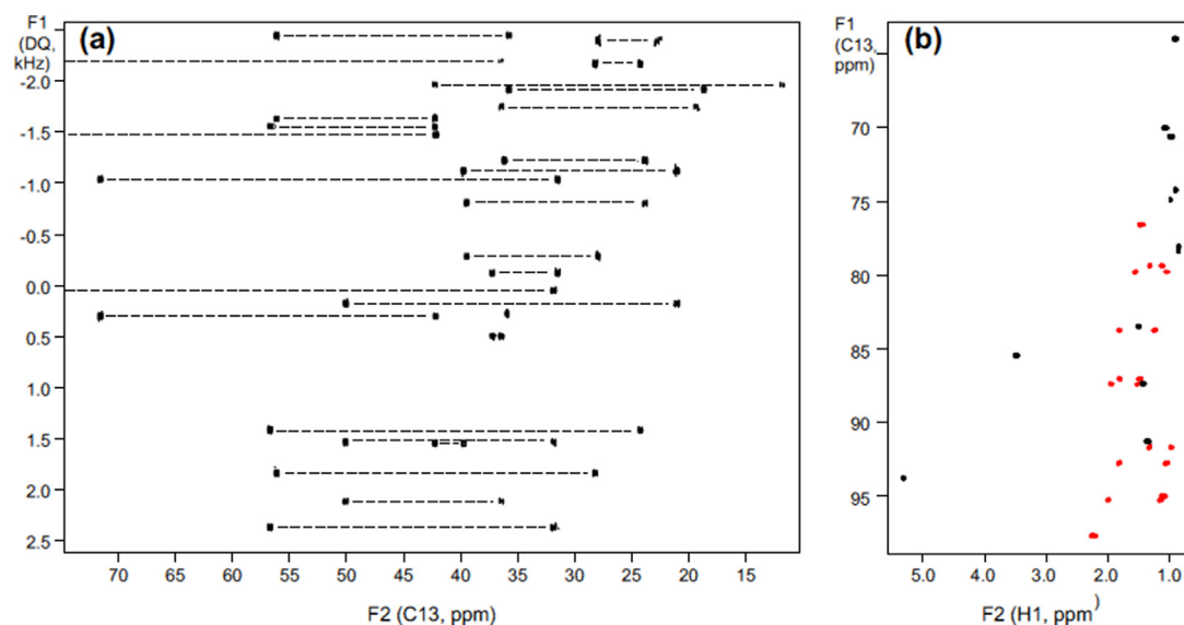
Fig. 34. The PANACEA spectra of 1 M cholesterol in CDCl 3 recorded in 23-min; a) 2D 13 C- 13 C INADEQUATE spectrum recorded with four-fold folding, b) multiplicity-edited HSQC spectrum; negative (red) peaks belong to CH 2 groups and black peaks represent CH and CH 3 groups. Reproduced from Ref. [114] with permission.
