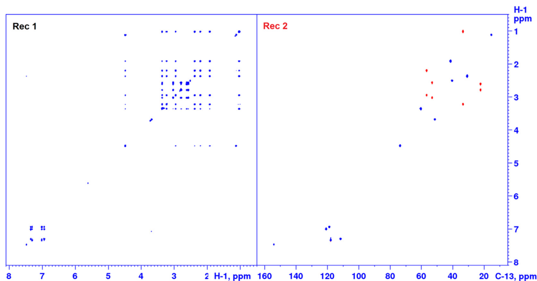
Fig. 22. TOCSY (receiver 1) and 2D multiplicity edited ^1\text{H} - ^{13}\text{C} HETCOR (receiver 2) spectra of ajmalicine in \text{DMSO-}d_6 (10 mg/600 \mu\text{l} ) recorded on a Bruker NEO 800 MHz instrument in 12 min using the pulse sequence of Fig. 21a; 256 increments, 2 scans per increment; negative \text{CH}_2 peaks in the HETCOR spectra are shown in red, positive (CH and \text{CH}_3 ) peaks are shown in blue.
