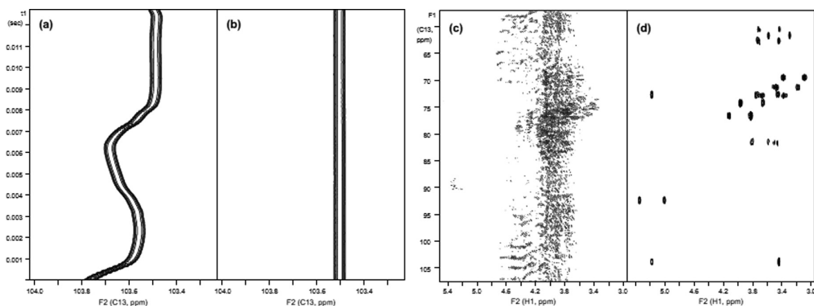
Fig. 32. (a) Instabilities due to disabled deuterium field/frequency lock and temperature regulation as detected in 1D ^{13}C spectra of 1 M sucrose in D_2O recorded with the PANACEA pulse scheme of Fig. 31a. (b) The corrected 1D ^{13}C spectrum; (c) the corrupted PANACEA-HMBC spectrum without ^2H lock and temperature regulation; (d) the same spectrum following post-acquisition field/frequency correction using the 1D ^{13}C spectrum. Reproduced from Ref. [114] with permission.
