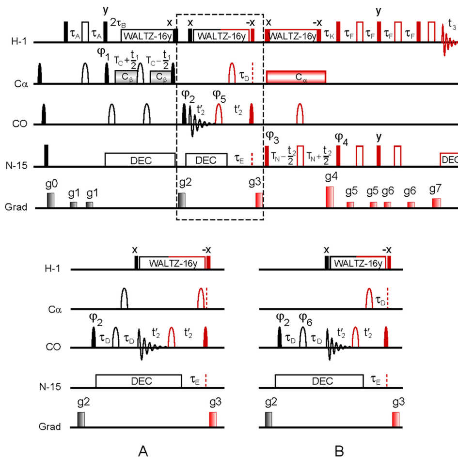
Fig. 40. Pulse scheme for recording 2D (HA)CACO (black)/3D (HA)CA(CO)NNH (black + red) with sequential detection of ^{13}\text{C} O and ^1\text{H} N FIDs. The antiphase doublet CO peaks in F2' are "collapsed" to singlets using the IPAP scheme - the dashed box is replaced by panels A and B in alternate scans. Delays: \tau_A = 1.7 ms, \tau_B = 1.8 ms, \tau_D = 4.625 ms, \tau_E = 24 ms, \tau_F = 2.3 ms, \tau_K = 5.5 ms, \tau_C = 4 ms, T_N = 12.4 ms. Phase cycling: \phi_1 = x, -x ; \phi_2 = 2(x), 2(-x) ; \phi_3 = 4(x), 4(-x) ; \phi_4 = x ; \text{Rec}^{(13\text{C})} = x, -x, -x, x ; \text{Rec}^{(1\text{H})} = x, 2(-x), x, -x, 2(x), -x . Phases \phi_5 (top scheme), \phi_6 (scheme B) are adjusted to compensate for Bloch-Siegert phase shifts introduced by the \text{C}\alpha pulse. Quadrature detection in F_1 is achieved by incrementing \phi_1 by 90^\circ . Quadrature detection in F_2 is achieved by recording a pair of data sets for each t_2 point with (g_4, \phi_4) and (-g_4, -\phi_4) . To apply the IPAP scheme sequence, A is implemented for (g_4, \phi_4) , and scheme B for (-g_4, -\phi_4) , thereby reducing the experiment time by a factor of two. Gradient pulses (G/cm, ms): g_0 = (10, 0.5) , g_1 = (8, 0.5) , g_2 = (20, 1) , g_3 = (-15, 1) , g_4 = (30, 1.25) , g_5 = (3, 0.3) , g_6 = (2.5, 0.4) , g_7 = (29.5, 0.125) . Reproduced from Ref. [138] with permission.
