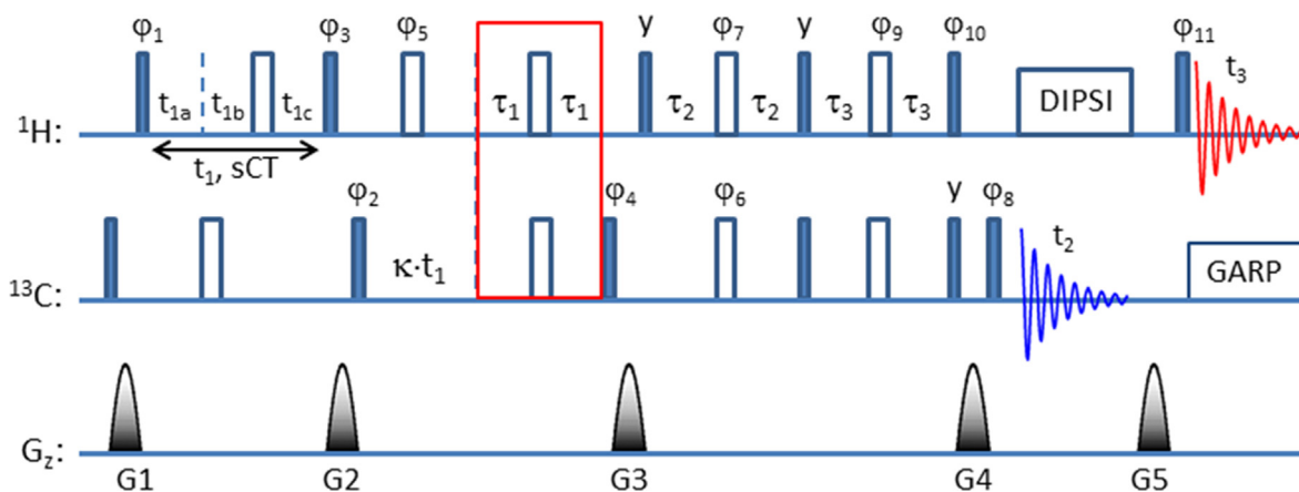
Fig. 50. Multiplicity-edited ^{13}\text{C} (3, 2)D HSQC-TOCSY / HETCOR / TOCSY pulse sequence [156]. All pulses are applied with phase 'x' unless indicated otherwise; phase cycling: \phi_1 = \phi_2 = x (incremented according to the States method); \phi_3 = y, -y ; \phi_4 = \phi_7 = \phi_{10} = x, -x ; \phi_4 is alternated for TS encoding; \phi_5 = \phi_6 = \phi_8 = \phi_9 = \phi_{11} = x, x, -x, -x ; \text{Rec}(^{13}\text{C}) = x, x, -x, -x ; \text{Rec}(^1\text{H}) = x, -x, -x, x . Delays: \tau_1 = 3.6 ms, \tau_2 = 1.79 ms, \tau_3 = 0.893 ms; the ^1\text{H} t_1 -evolution period is implemented in a semi-constant time manner; at t_1 = 0 the delays t_{1a} , t_{1b} and t_{1c} are set to 0.9 ms, 3 \mu\text{s} and 0.9 ms, respectively such that T_{\text{CT}} = t_{1a} + t_{1b} + t_{1c} = 0.25/|J(^{13}\text{C}-^1\text{H})| . The ^{13}\text{C} t_1 -evolution period is co-incremented with that of ^1\text{H} with a relative scaling factor ( \kappa ). The DIPSI mixing time was 80 ms. Gradient pulses (1 ms): G1 = G2 = G3 = G4 = 19 G/cm, G5 = 11 G/cm; the red box indicates an optional ^{13}\text{C} multiplicity editing block.
