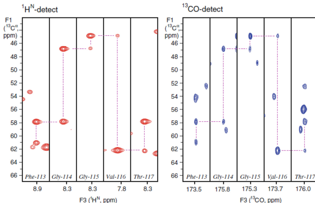
Fig. 46. F_1F_3 strip plots of ^1\text{H} - (left) and ^{13}\text{CO} - (right) detected 3D HNCA spectra of 1 mM Lb-FABP protein (9:1 \text{H}_2\text{O}/\text{D}_2\text{O} , 25^\circ\text{C} ), recorded using the pulse scheme of Fig. 45 on an Agilent 800 MHz DDR2 NMR system equipped with two receivers and a cryogenic ^{13}\text{C} and ^1\text{H} sensitivity-enhanced probe. The ^1J(^{13}\text{C}\alpha\text{--}^{13}\text{CO}) coupling was suppressed using the IPAP scheme. The total experiment time was 11 h 20 min. Reproduced from Ref. [107] with permission.
