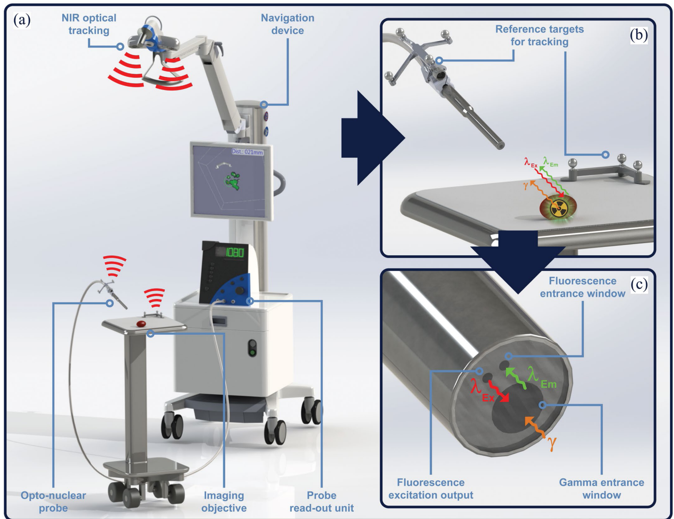
Fig. 1. Schematic overview of the hybrid imaging and navigation modality. (a) Overview of the total setup, showing near-infrared (NIR) tracking of both the opto-nuclear probe and the imaging objective. (b) Zoom-in of the opto-nuclear probe and imaging objective, displaying the presence of both a radioactive ( \gamma ) and fluorescent ( \lambda_{\text{Excitation}} and \lambda_{\text{Emission}} ) tracer signature in the imaging objective. (c) Zoom-in of the probe entrance windows for nuclear and fluorescence detection.
