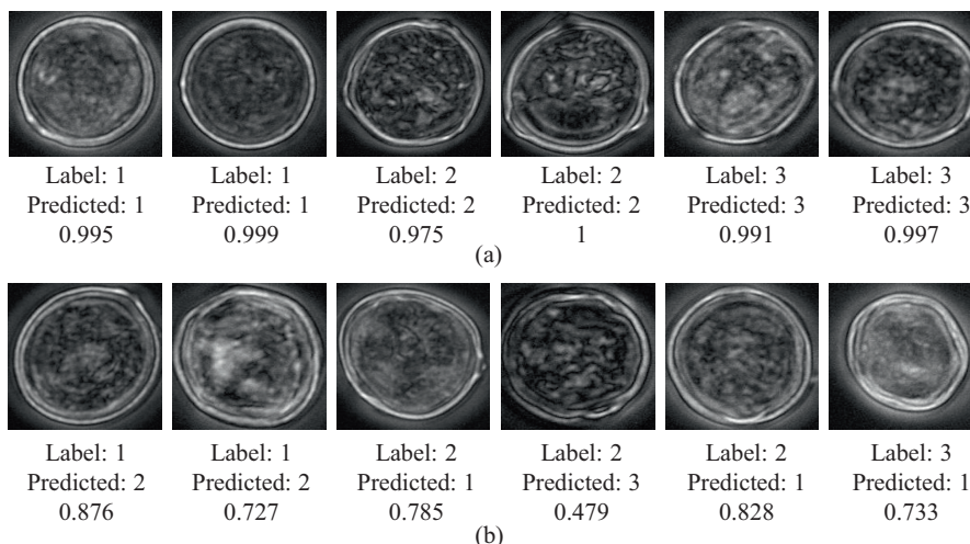
Fig. 6. Examples of classification performed by VGG16. (a) Positive samples with their predicted label and confidence score. (b) Negative samples with their predicted label and confidence score.
