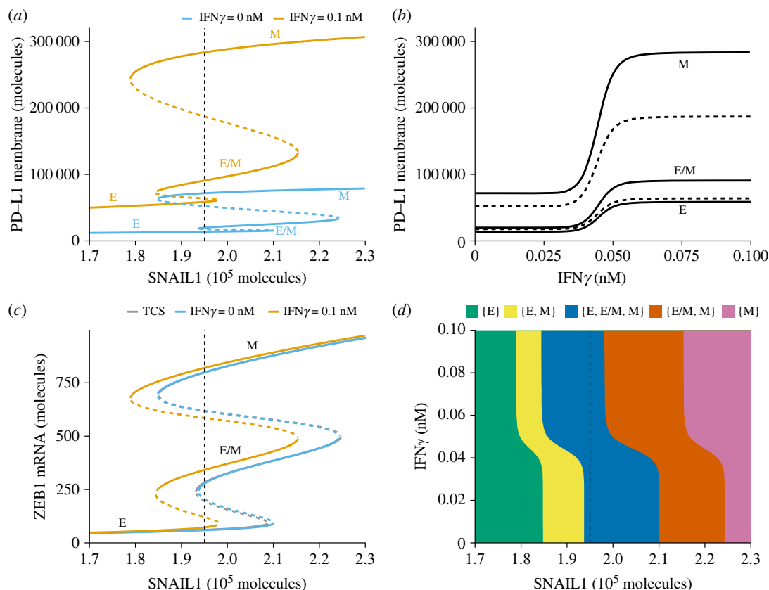
Figure 2. Model-predicted mutual influence of IFN \gamma -driven PD-L1 expression and EMT. (a–c) Bifurcation (a,c) and continuation (b) diagrams illustrating how the steady-state expression of PD-L1 on the membrane depends on SNAIL1 in the absence (blue) and presence (orange) of IFN \gamma (a), how the steady-state expression of PD-L1 on the membrane depends on IFN \gamma , considering a fixed SNAIL1 level of 1.95 \times 10^5 molecules (b) and how the steady state of ZEB1 mRNA depends on SNAIL1 in the TCS model (grey), and in our extended model in the absence (blue) or presence (orange) of IFN \gamma (c). Stable equilibria (representing E, E/M and M phenotypes) are indicated by solid lines and unstable equilibria by dashed lines. (d) Phase diagram showing how the presence of stable equilibria (coloured regions, indicated in the legend) depends on IFN \gamma and SNAIL1. Vertical dashed lines in (a), (c) and (d) show the SNAIL1 concentration used in (b).
