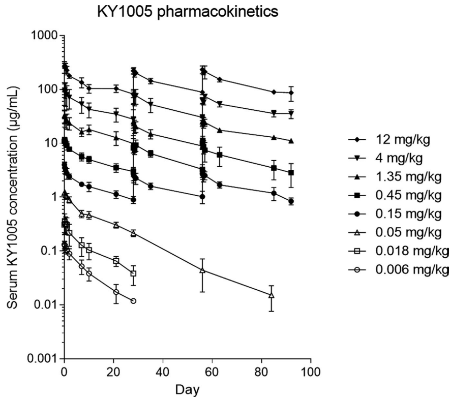
Figure 2 KY1005 serum concentrations ( \mu\text{g/mL} ). Data displayed on log10 scale as mean (SD).
