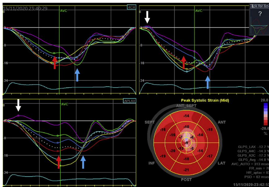
Figure 16. Strain in a patient with LAD infarct. Typical strain patterns in acute myocardial ischemia are early systolic lengthening (white arrows), reduced systolic strain (red arrows), and post-systolic shortening (blue arrows). The bull-eye plot contains areas with lighter colors which indicate LV segments with decreased function.
