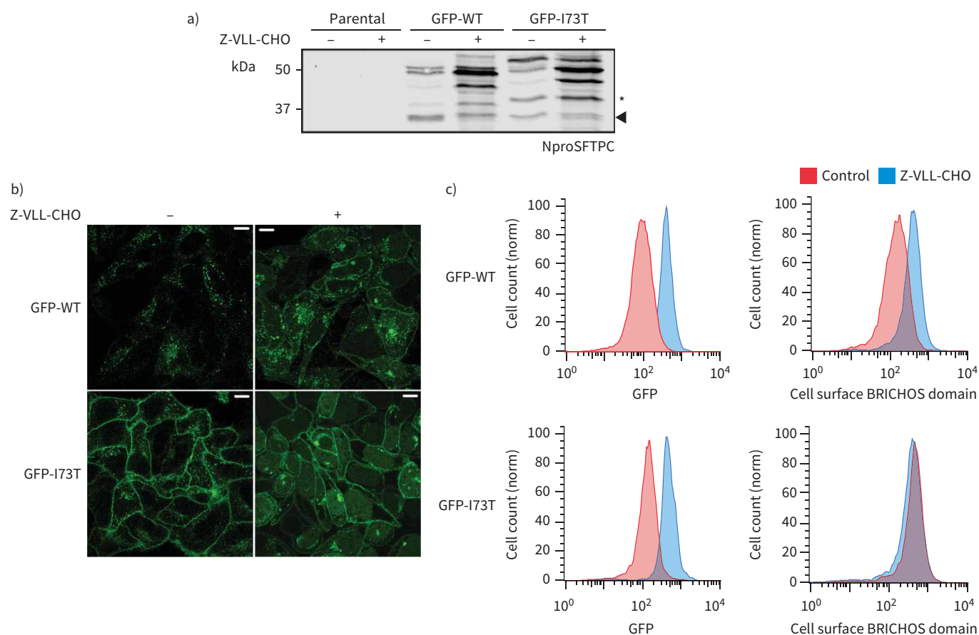
FIGURE 7 Surfactant protein C (SFTPC) C-terminal cleavage is inhibited by Z-VLL-CHO. a) HeLa cells stably expressing green fluorescent protein (GFP)-SFTPC-wild type (WT) or -I73T were treated with 5 \mu M Z-VLL-CHO for 16 h and lysates immunoblotted for NproSFTPC. Cells treated with Z-VLL-CHO develop an excess of early C-terminal processing intermediates, increased overall SFTPC (as measured by GFP) and redistribution of SFTPC to the plasma membrane, as seen by b) confocal microscopy and c) flow cytometry. Scale bar=10 \mu m.
