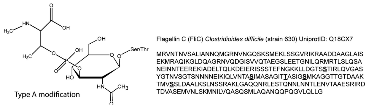
Figure 1. Structure of the type A modification of Clostridioides difficile strain 630 \Delta erm flagellin C (FliC). Left , structure of the type A modification consisting of an O-linked GlcNAc, linked, through a phosphodiester, to an N-methyl-L-threonine. Right , type A-modified serine and threonine residues of C. difficile strain 630 FliC (UniProt ID: Q18CX7), bold and underlined . Based on Faulds-Pain et al. (19) and Twine et al. (15).
